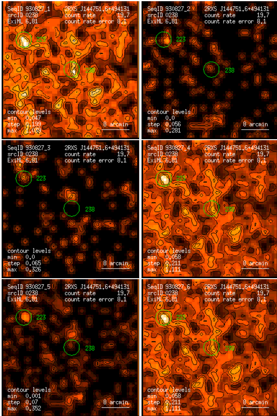
Figure 238: RASS 930827: detection 0238: band rate images, Gaussian filter: (1) PSPC channels 11 – 41, (2) 52 – 90, (3) 91 – 201, (4) 11 – 235, (5) 52 – 201, (6) 11 – 201. Broad band rates in counts/ks. Band rate contour levels in counts/ks/arcmin 2 .
