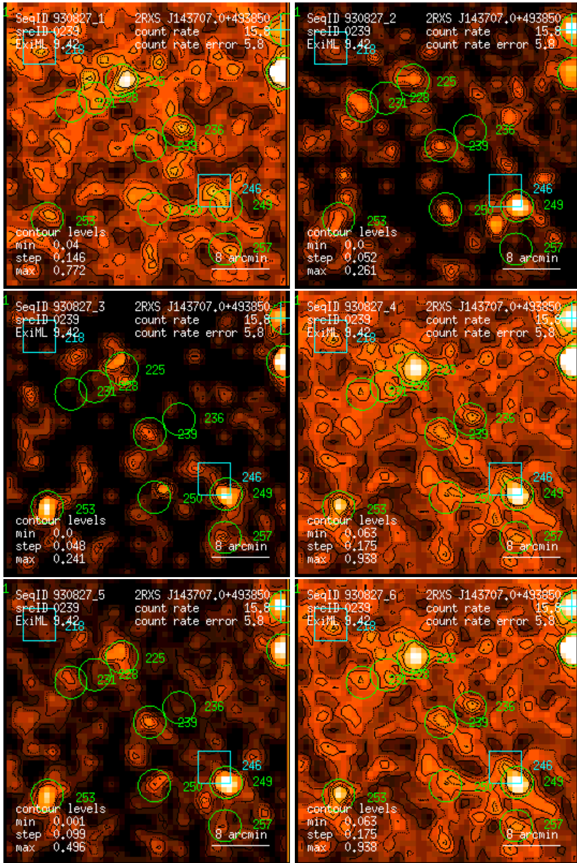
Figure 239: RASS 930827: detection 0239: band rate images, Gaussian filter: (1) PSPC channels 11 – 41, (2) 52 – 90, (3) 91 – 201, (4) 11 – 235, (5) 52 – 201, (6) 11 – 201. Broad band rates in counts/ks. Band rate contour levels in counts/ks/arcmin 2 .
