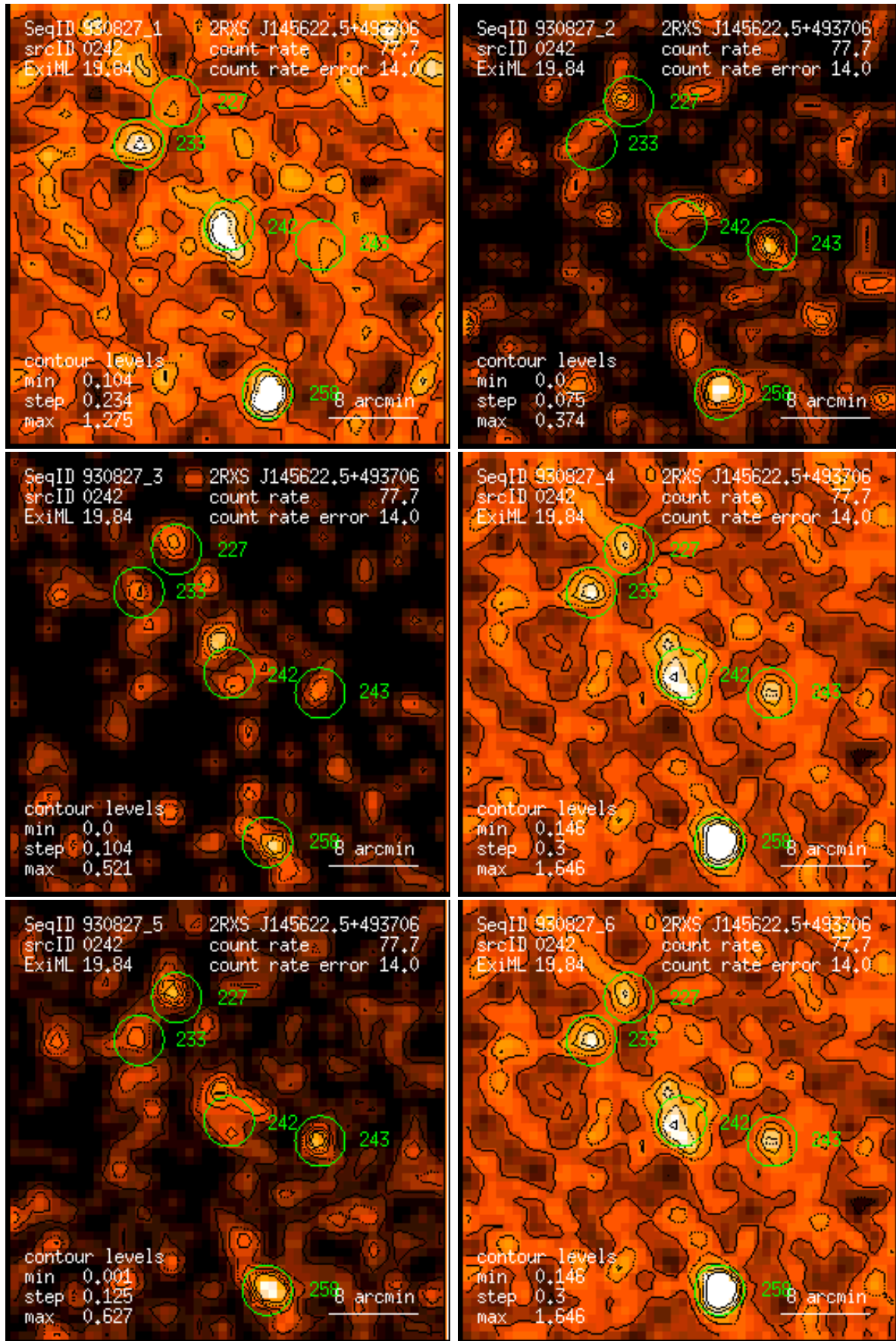
Figure 242: RASS 930827: detection 0242: band rate images, Gaussian filter: (1) PSPC channels 11 – 41, (2) 52 – 90, (3) 91 – 201, (4) 11 – 235, (5) 52 – 201, (6) 11 – 201. Broad band rates in counts/ks. Band rate contour levels in counts/ks/arcmin 2 .
