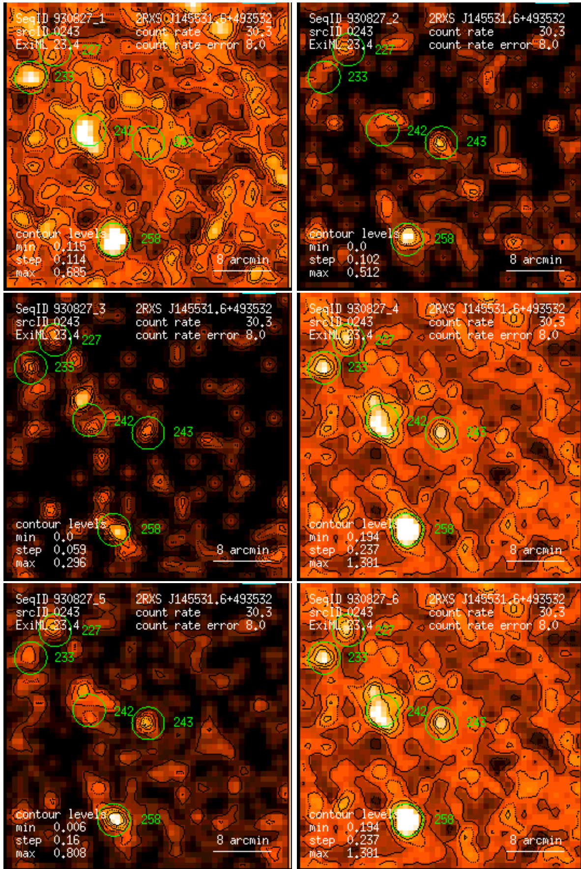
Figure 243: RASS 930827: detection 0243: band rate images, Gaussian filter: (1) PSPC channels 11 – 41, (2) 52 – 90, (3) 91 – 201, (4) 11 – 235, (5) 52 – 201, (6) 11 – 201. Broad band rates in counts/ks. Band rate contour levels in counts/ks/arcmin 2 .
