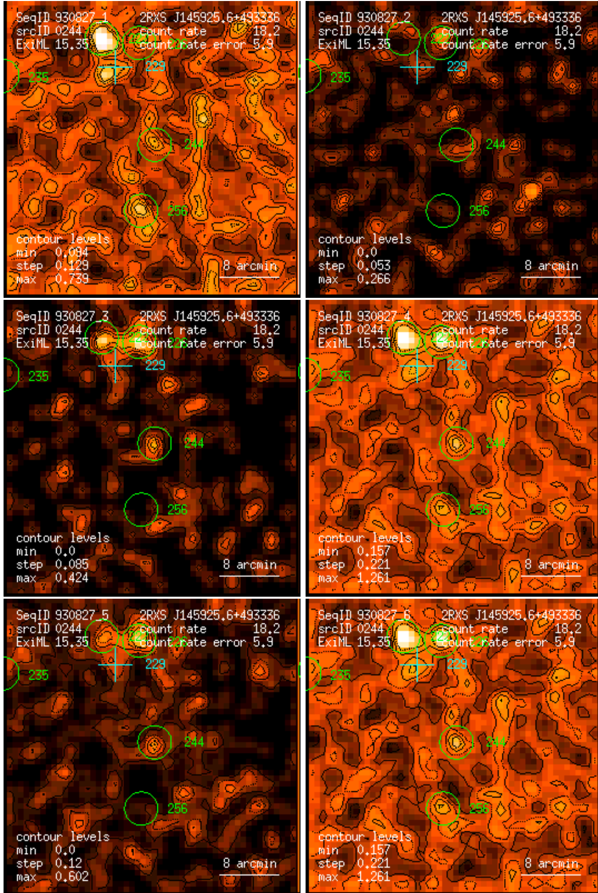
Figure 244: RASS 930827: detection 0244: band rate images, Gaussian filter: (1) PSPC channels 11 – 41, (2) 52 – 90, (3) 91 – 201, (4) 11 – 235, (5) 52 – 201, (6) 11 – 201. Broad band rates in counts/ks. Band rate contour levels in counts/ks/arcmin 2 .
