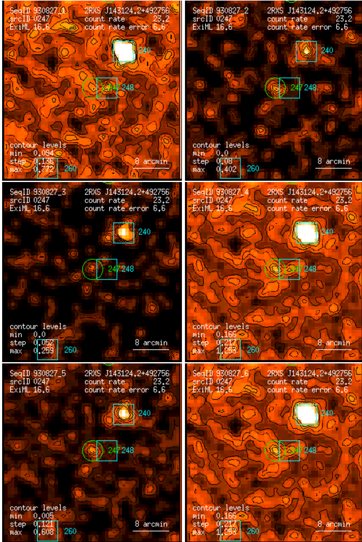
Figure 247: RASS 930827: detection 0247: band rate images, Gaussian filter: (1) PSPC channels 11 – 41, (2) 52 – 90, (3) 91 – 201, (4) 11 – 235, (5) 52 – 201, (6) 11 – 201. Broad band rates in counts/ks. Band rate contour levels in counts/ks/arcmin 2 .
