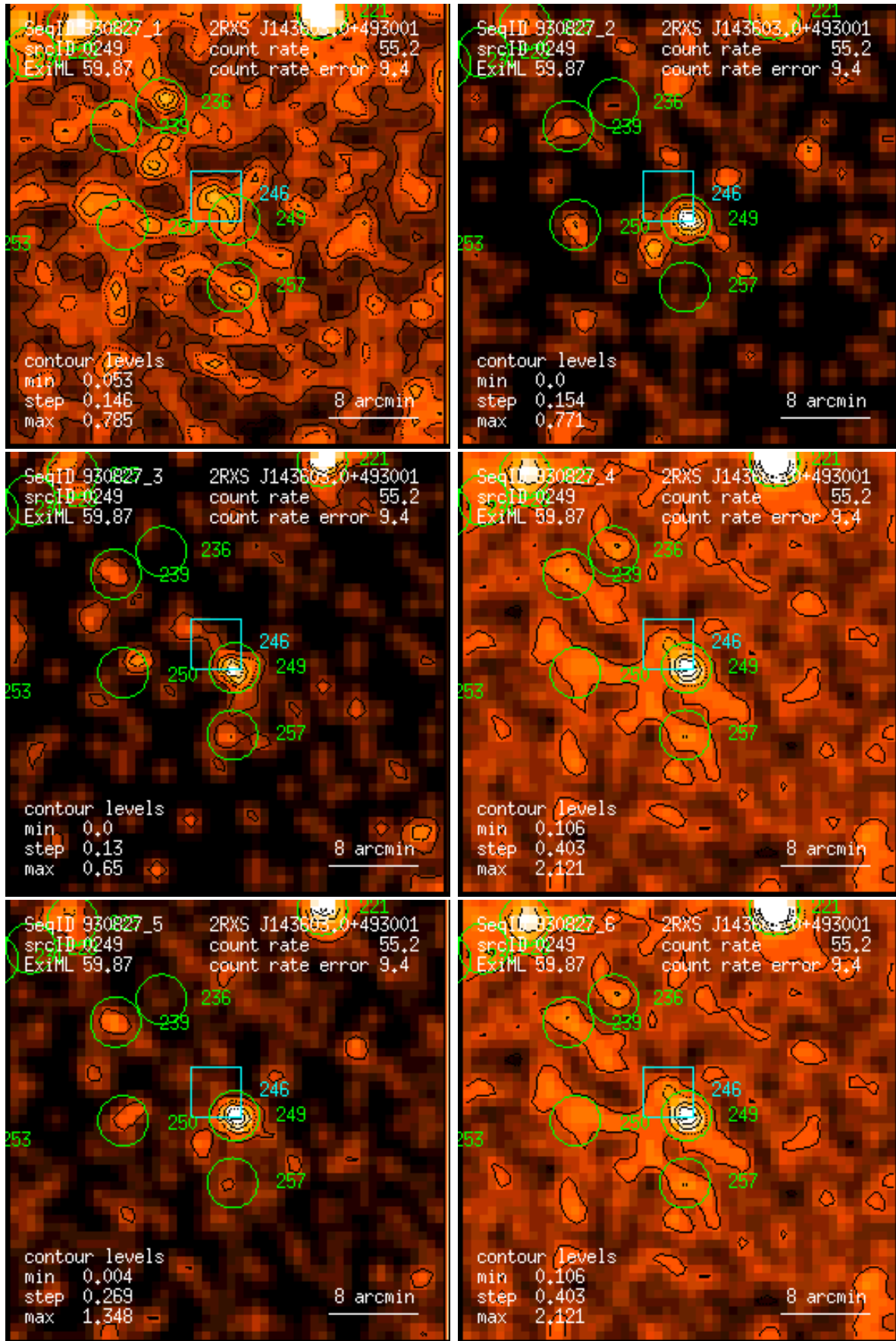
Figure 249: RASS 930827: detection 0249: band rate images, Gaussian filter: (1) PSPC channels 11 – 41, (2) 52 – 90, (3) 91 – 201, (4) 11 – 235, (5) 52 – 201, (6) 11 – 201. Broad band rates in counts/ks. Band rate contour levels in counts/ks/arcmin 2 .
