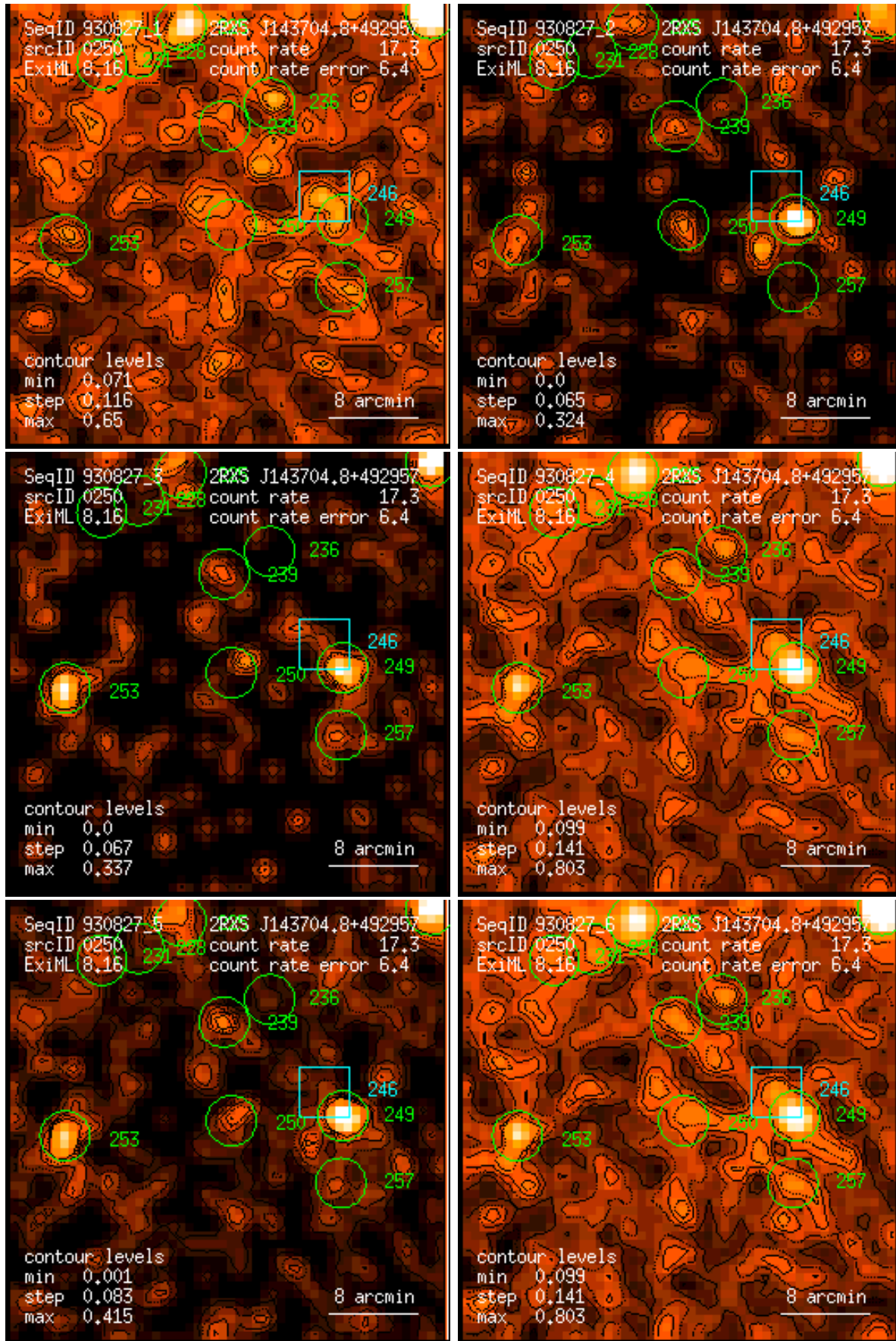
Figure 250: RASS 930827: detection 0250: band rate images, Gaussian filter: (1) PSPC channels 11 – 41, (2) 52 – 90, (3) 91 – 201, (4) 11 – 235, (5) 52 – 201, (6) 11 – 201. Broad band rates in counts/ks. Band rate contour levels in counts/ks/arcmin 2 .
