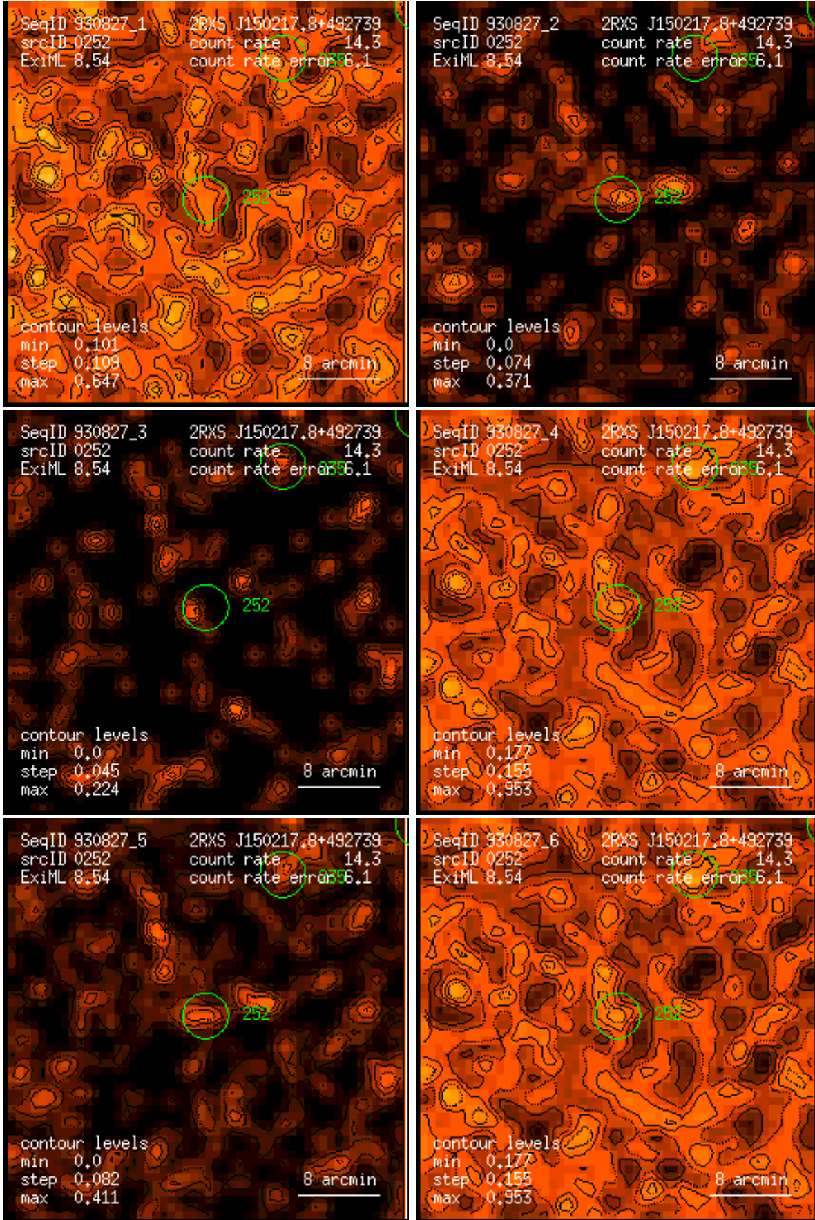
Figure 252: RASS 930827: detection 0252: band rate images, Gaussian filter: (1) PSPC channels 11 – 41, (2) 52 – 90, (3) 91 – 201, (4) 11 – 235, (5) 52 – 201, (6) 11 – 201. Broad band rates in counts/ks. Band rate contour levels in counts/ks/arcmin 2 .
