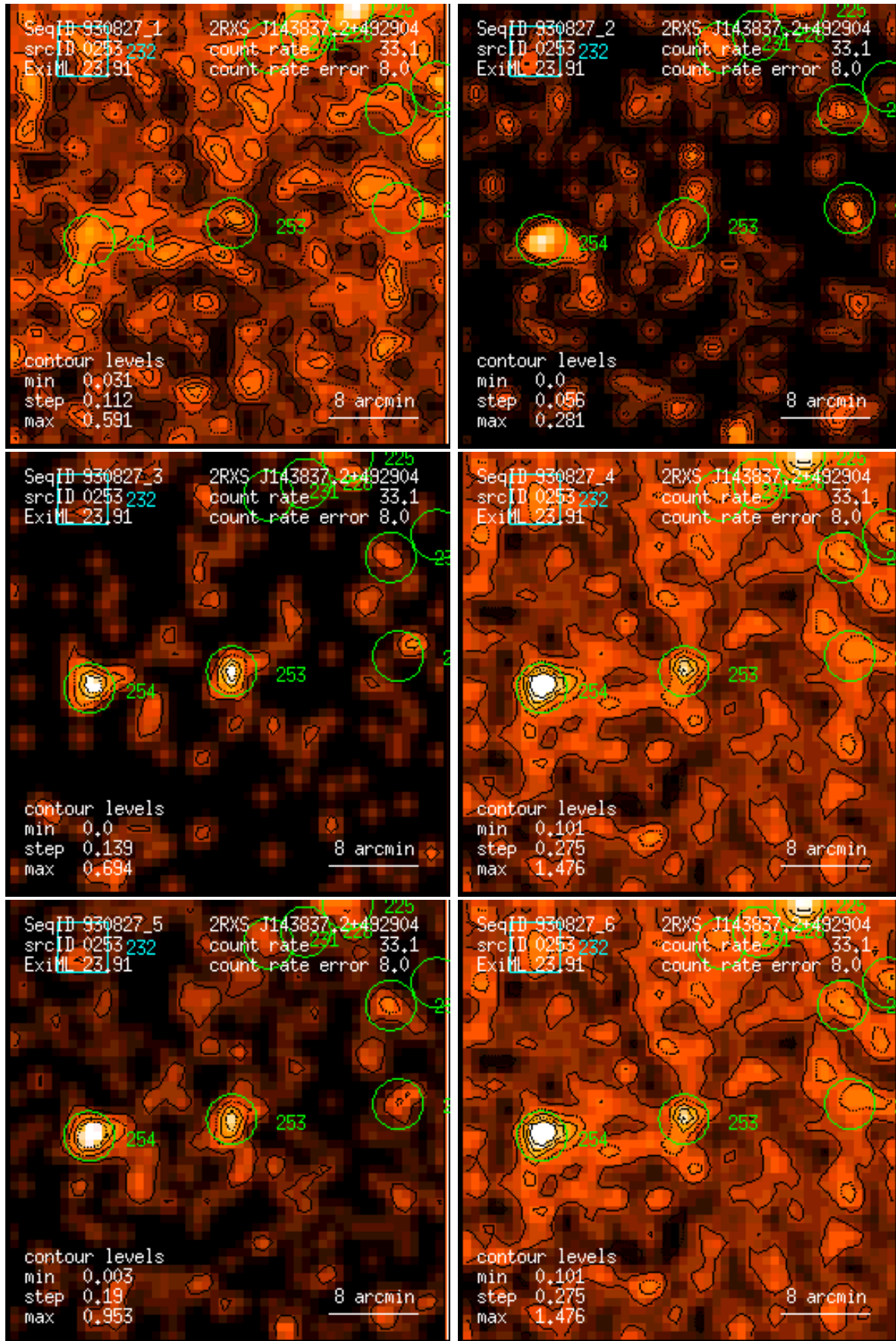
Figure 253: RASS 930827: detection 0253: band rate images, Gaussian filter: (1) PSPC channels 11 – 41, (2) 52 – 90, (3) 91 – 201, (4) 11 – 235, (5) 52 – 201, (6) 11 – 201. Broad band rates in counts/ks. Band rate contour levels in counts/ks/arcmin 2 .
