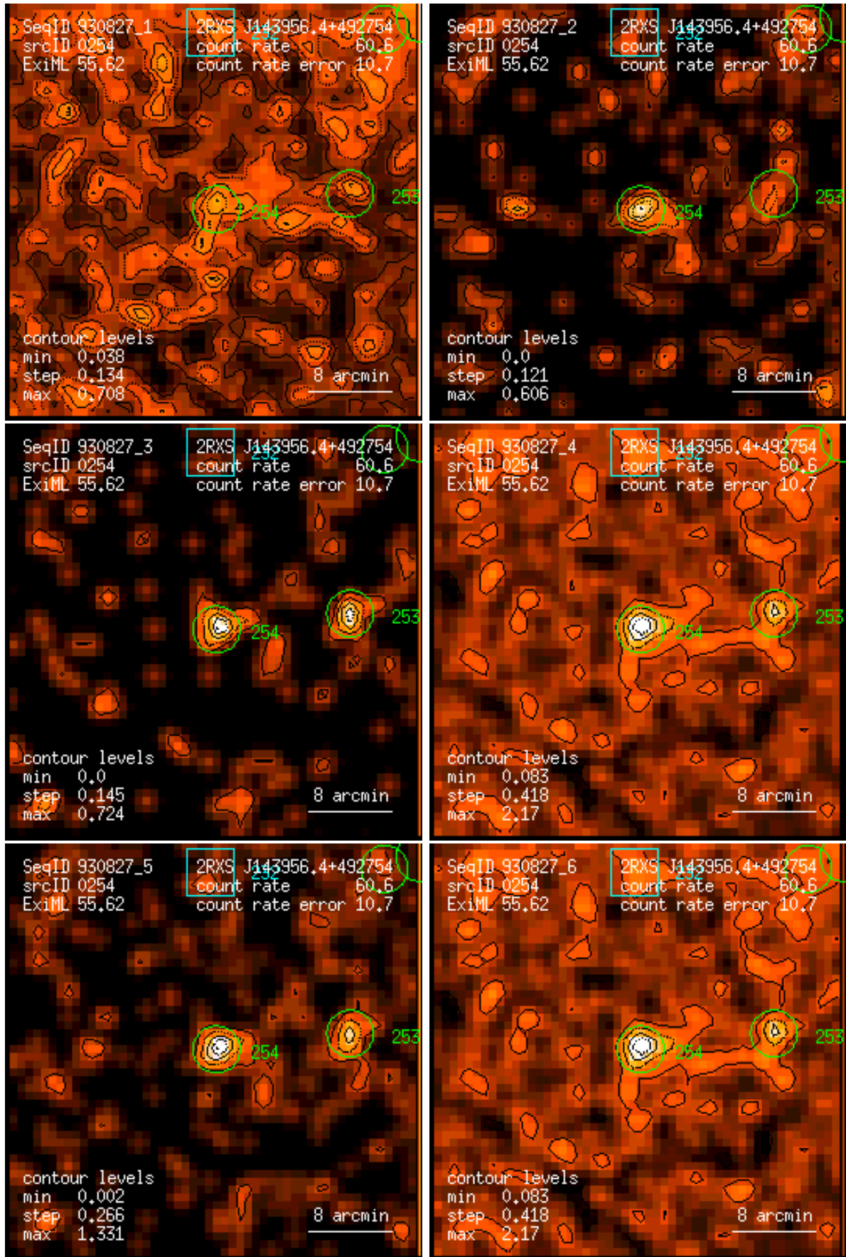
Figure 254: RASS 930827: detection 0254: band rate images, Gaussian filter: (1) PSPC channels 11 – 41, (2) 52 – 90, (3) 91 – 201, (4) 11 – 235, (5) 52 – 201, (6) 11 – 201. Broad band rates in counts/ks. Band rate contour levels in counts/ks/arcmin 2 .
