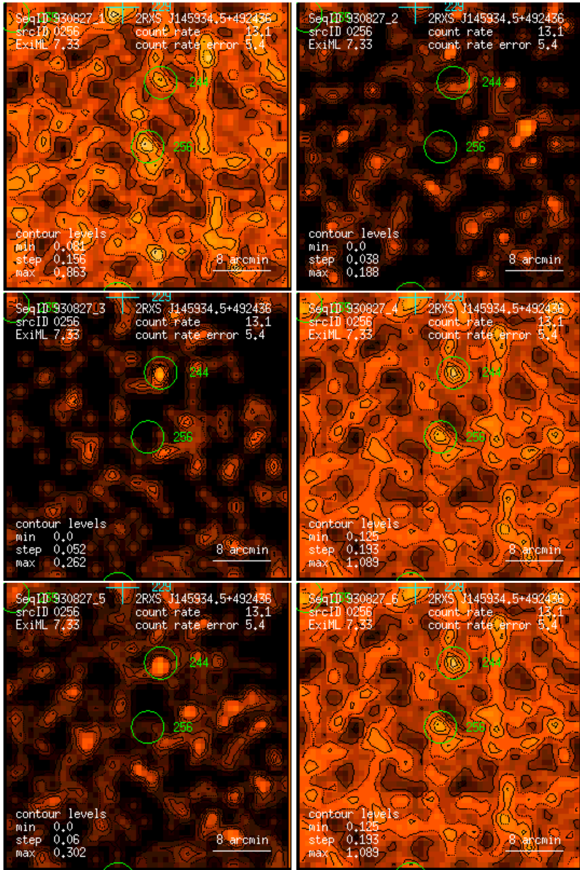
Figure 256: RASS 930827: detection 0256: band rate images, Gaussian filter: (1) PSPC channels 11 – 41, (2) 52 – 90, (3) 91 – 201, (4) 11 – 235, (5) 52 – 201, (6) 11 – 201. Broad band rates in counts/ks. Band rate contour levels in counts/ks/arcmin 2 .
