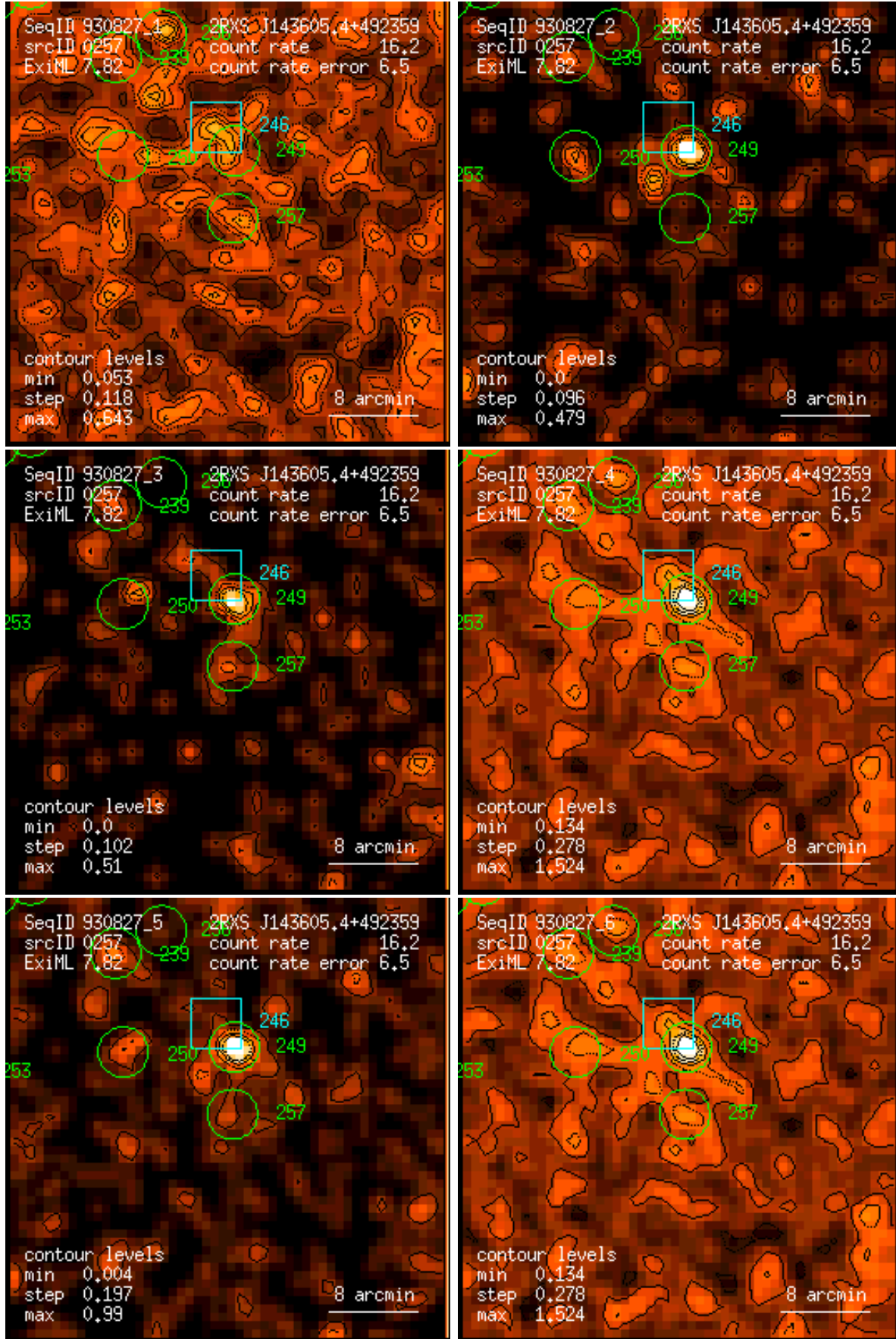
Figure 257: RASS 930827: detection 0257: band rate images, Gaussian filter: (1) PSPC channels 11 – 41, (2) 52 – 90, (3) 91 – 201, (4) 11 – 235, (5) 52 – 201, (6) 11 – 201. Broad band rates in counts/ks. Band rate contour levels in counts/ks/arcmin 2 .
