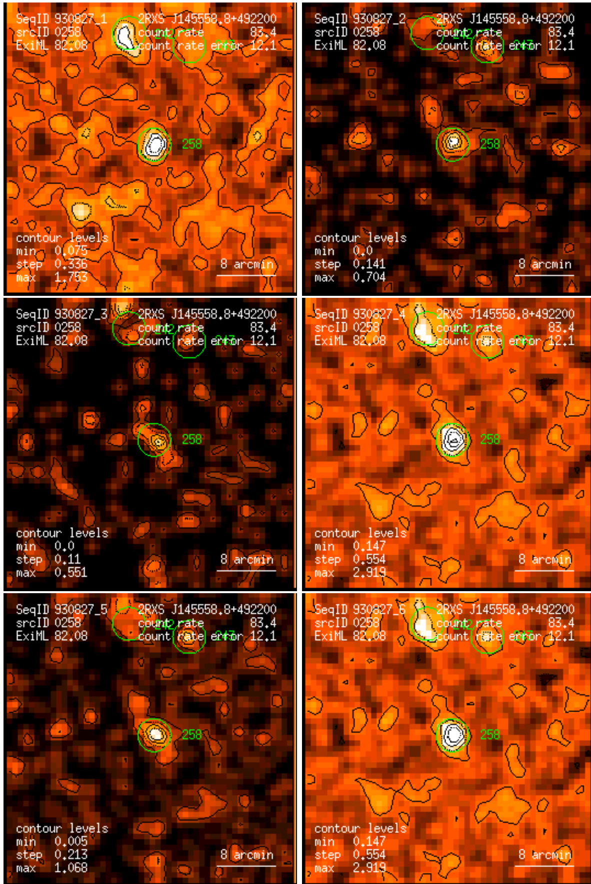
Figure 258: RASS 930827: detection 0258: band rate images, Gaussian filter: (1) PSPC channels 11 – 41, (2) 52 – 90, (3) 91 – 201, (4) 11 – 235, (5) 52 – 201, (6) 11 – 201. Broad band rates in counts/ks. Band rate contour levels in counts/ks/arcmin 2 .
