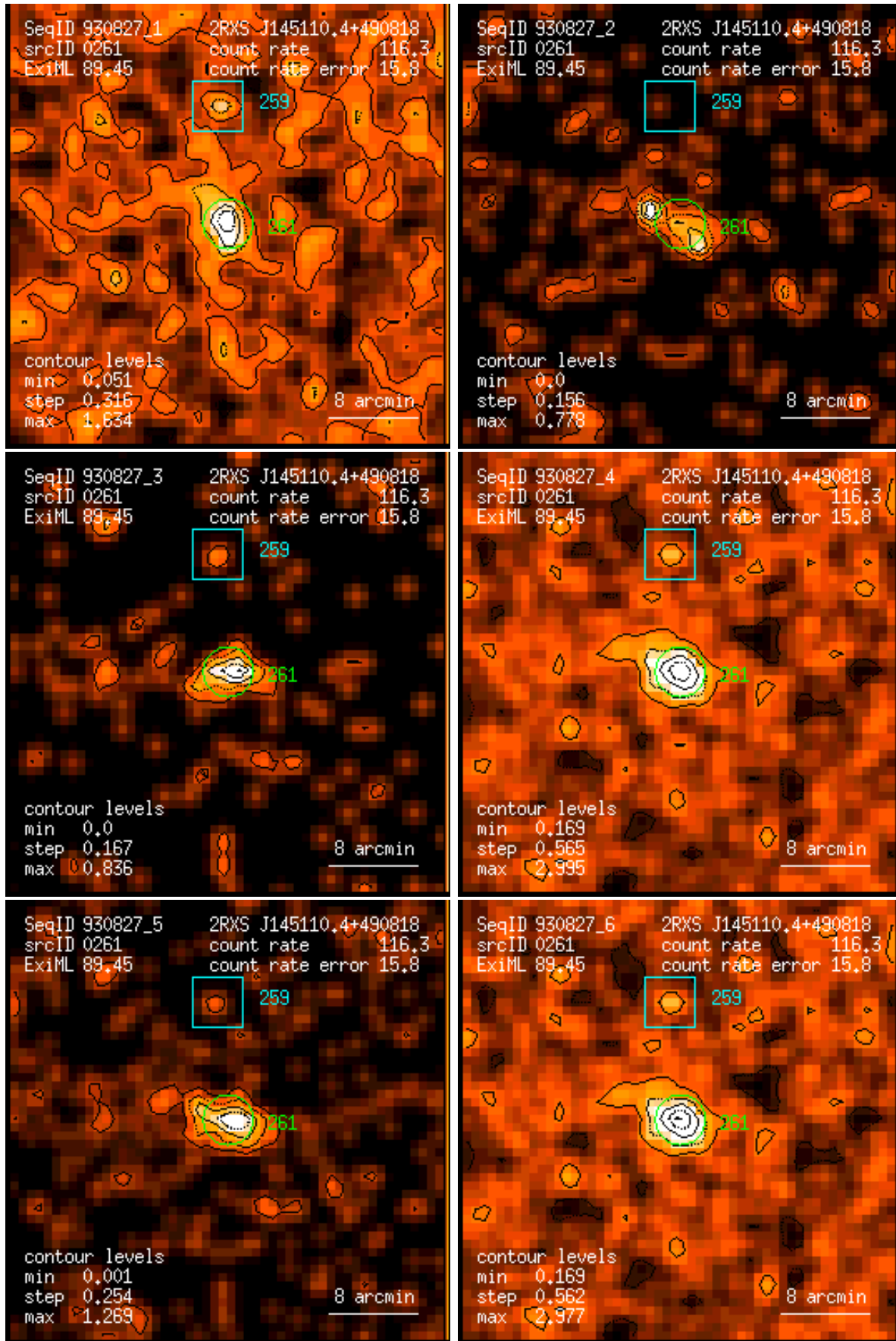
Figure 261: RASS 930827: detection 0261: band rate images, Gaussian filter: (1) PSPC channels 11 – 41, (2) 52 – 90, (3) 91 – 201, (4) 11 – 235, (5) 52 – 201, (6) 11 – 201. Broad band rates in counts/ks. Band rate contour levels in counts/ks/arcmin 2 .
