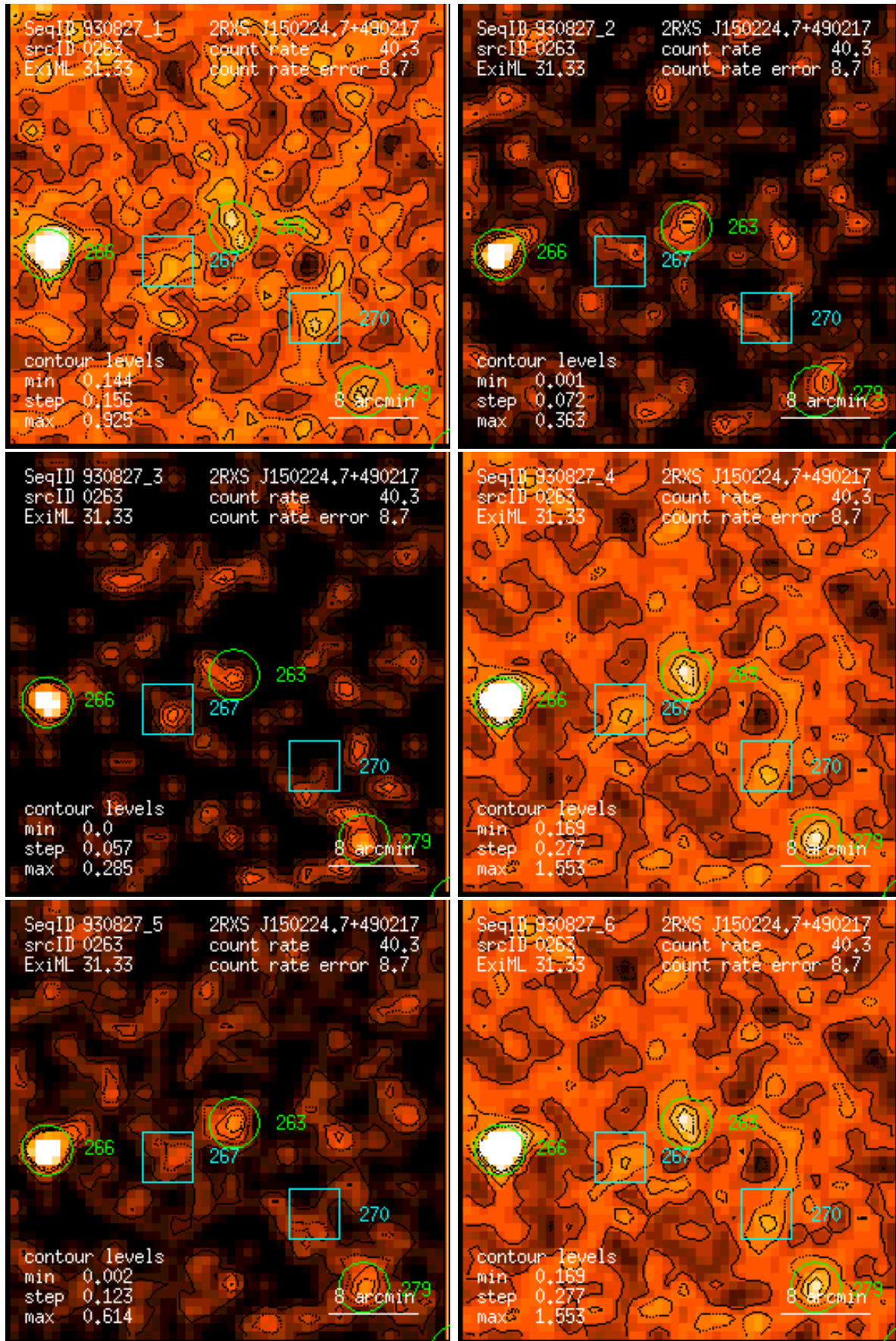
Figure 263: RASS 930827: detection 0263: band rate images, Gaussian filter: (1) PSPC channels 11 – 41, (2) 52 – 90, (3) 91 – 201, (4) 11 – 235, (5) 52 – 201, (6) 11 – 201. Broad band rates in counts/ks. Band rate contour levels in counts/ks/arcmin 2 .
