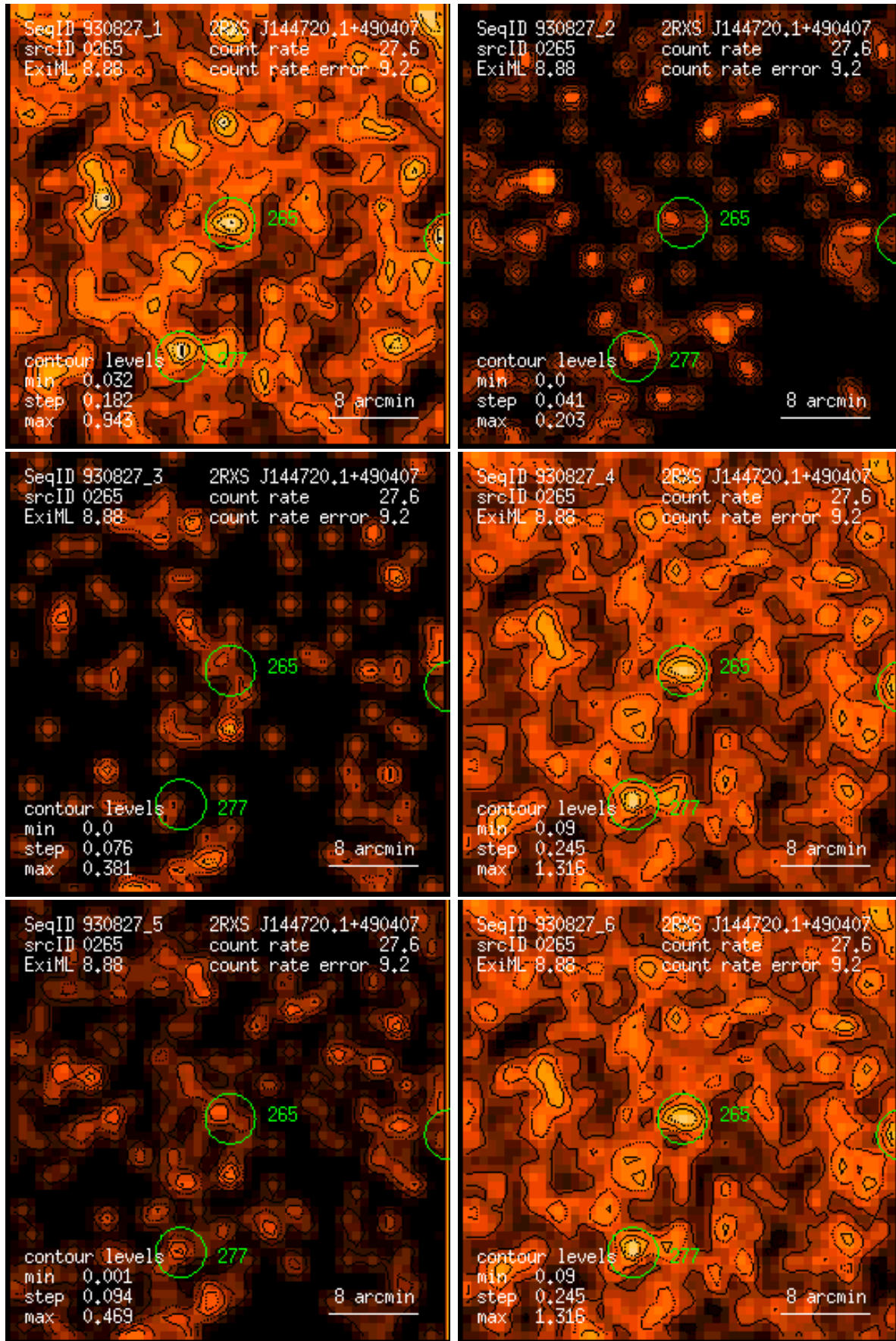
Figure 265: RASS 930827: detection 0265: band rate images, Gaussian filter: (1) PSPC channels 11 – 41, (2) 52 – 90, (3) 91 – 201, (4) 11 – 235, (5) 52 – 201, (6) 11 – 201. Broad band rates in counts/ks. Band rate contour levels in counts/ks/arcmin 2 .
