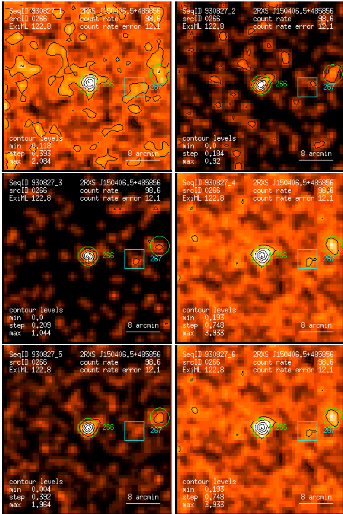
Figure 266: RASS 930827: detection 0266: band rate images, Gaussian filter: (1) PSPC channels 11 – 41, (2) 52 – 90, (3) 91 – 201, (4) 11 – 235, (5) 52 – 201, (6) 11 – 201. Broad band rates in counts/ks. Band rate contour levels in counts/ks/arcmin 2 .
