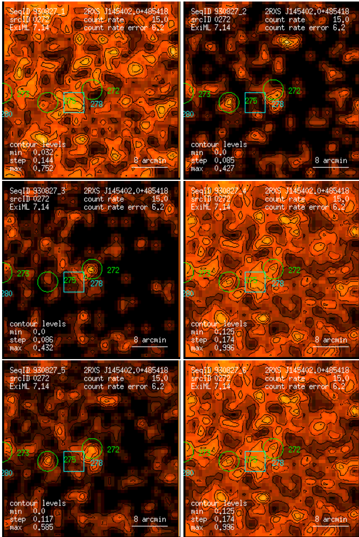
Figure 272: RASS 930827: detection 0272: band rate images, Gaussian filter: (1) PSPC channels 11 – 41, (2) 52 – 90, (3) 91 – 201, (4) 11 – 235, (5) 52 – 201, (6) 11 – 201. Broad band rates in counts/ks. Band rate contour levels in counts/ks/arcmin 2 .
