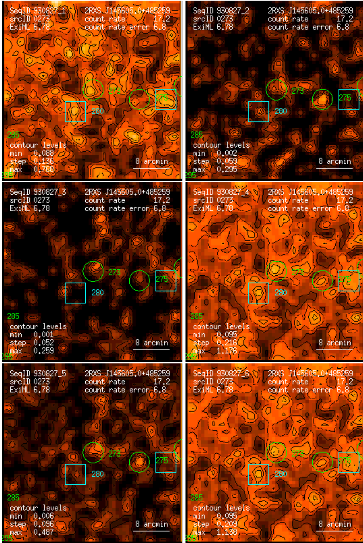
Figure 273: RASS 930827: detection 0273: band rate images, Gaussian filter: (1) PSPC channels 11 – 41, (2) 52 – 90, (3) 91 – 201, (4) 11 – 235, (5) 52 – 201, (6) 11 – 201. Broad band rates in counts/ks. Band rate contour levels in counts/ks/arcmin 2 .
