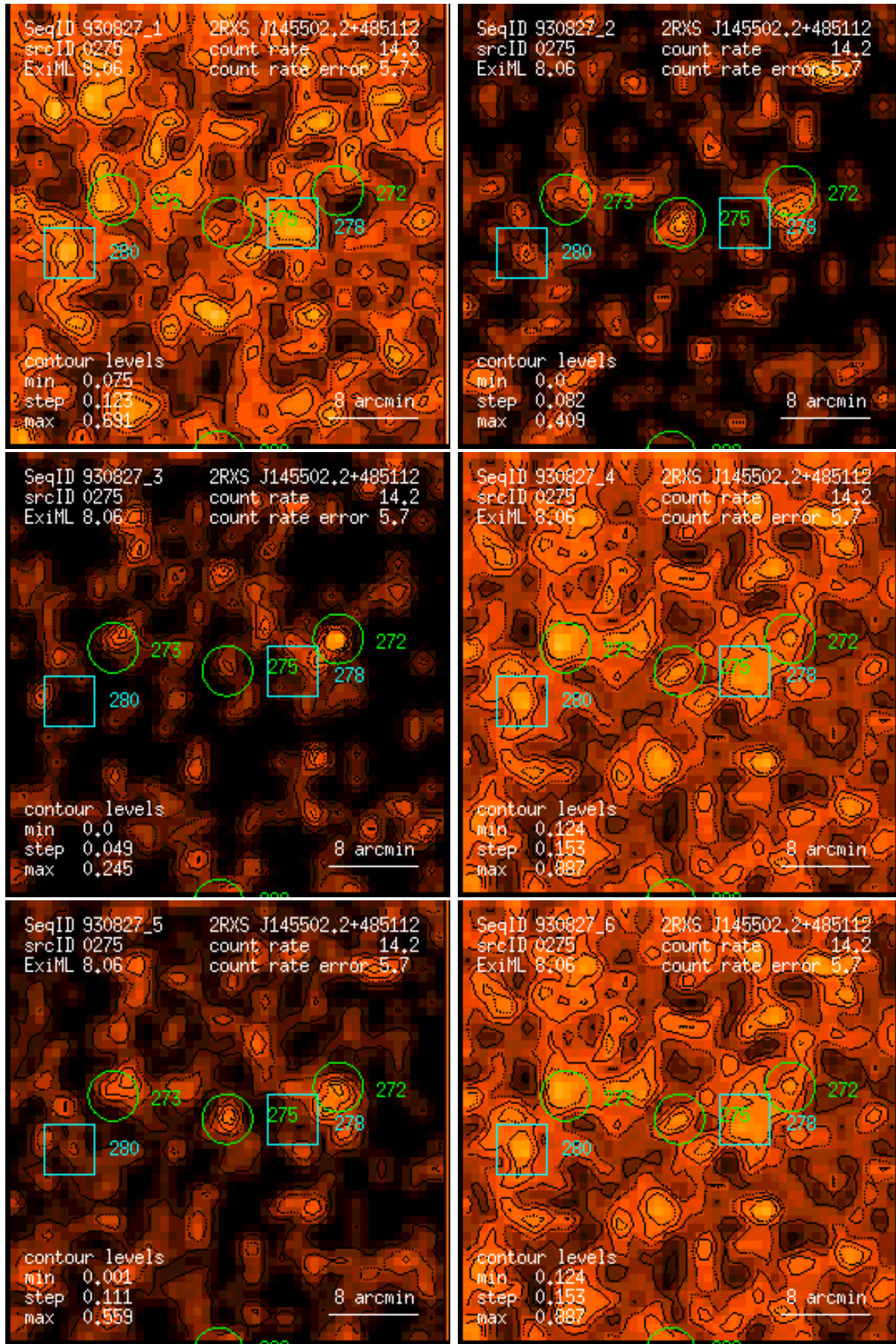
Figure 275: RASS 930827: detection 0275: band rate images, Gaussian filter: (1) PSPC channels 11 – 41, (2) 52 – 90, (3) 91 – 201, (4) 11 – 235, (5) 52 – 201, (6) 11 – 201. Broad band rates in counts/ks. Band rate contour levels in counts/ks/arcmin 2 .
