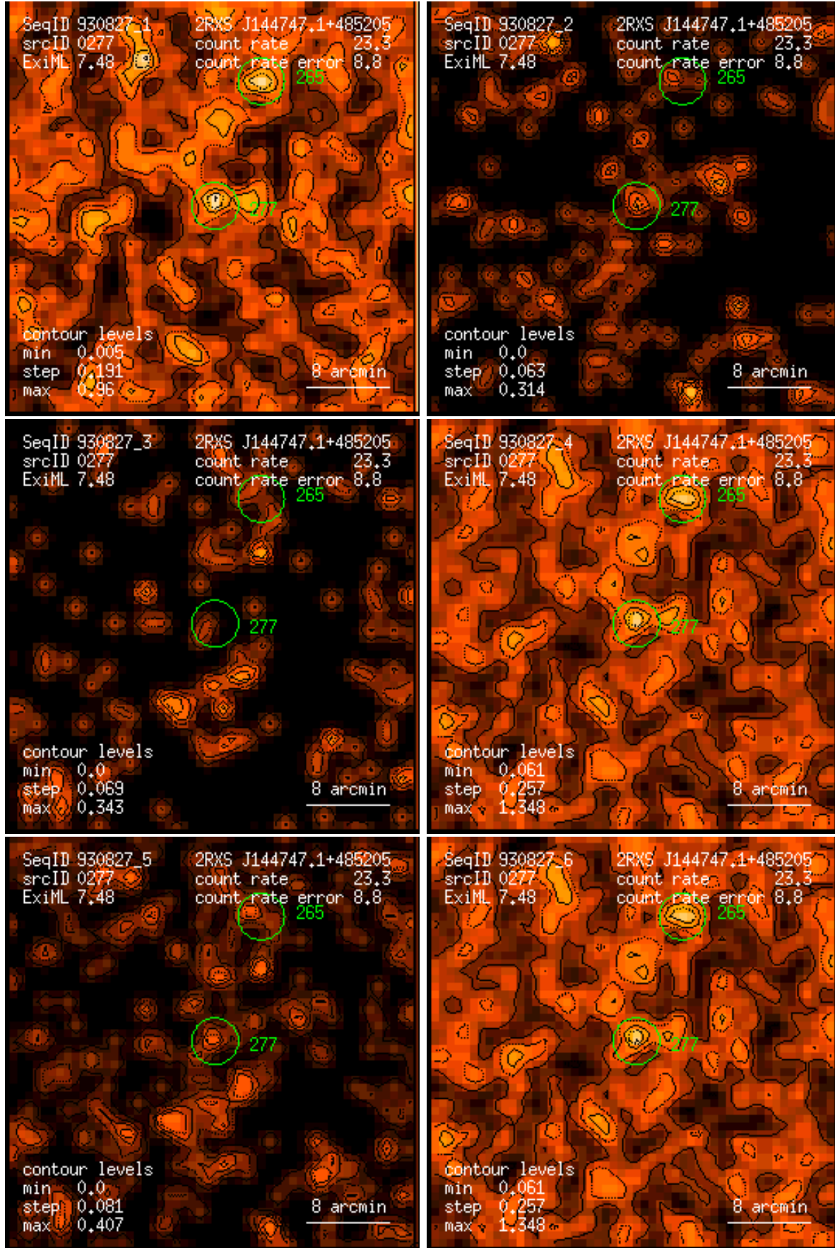
Figure 277: RASS 930827: detection 0277: band rate images, Gaussian filter: (1) PSPC channels 11 – 41, (2) 52 – 90, (3) 91 – 201, (4) 11 – 235, (5) 52 – 201, (6) 11 – 201. Broad band rates in counts/ks. Band rate contour levels in counts/ks/arcmin 2 .
