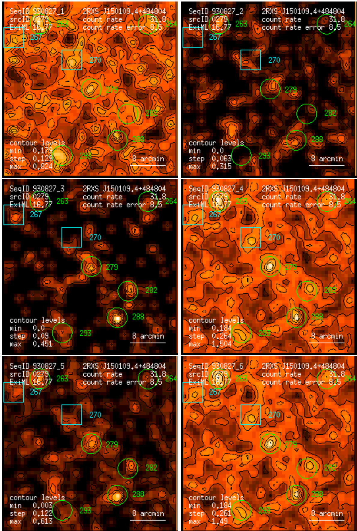
Figure 279: RASS 930827: detection 0279: band rate images, Gaussian filter: (1) PSPC channels 11 – 41, (2) 52 – 90, (3) 91 – 201, (4) 11 – 235, (5) 52 – 201, (6) 11 – 201. Broad band rates in counts/ks. Band rate contour levels in counts/ks/arcmin 2 .
