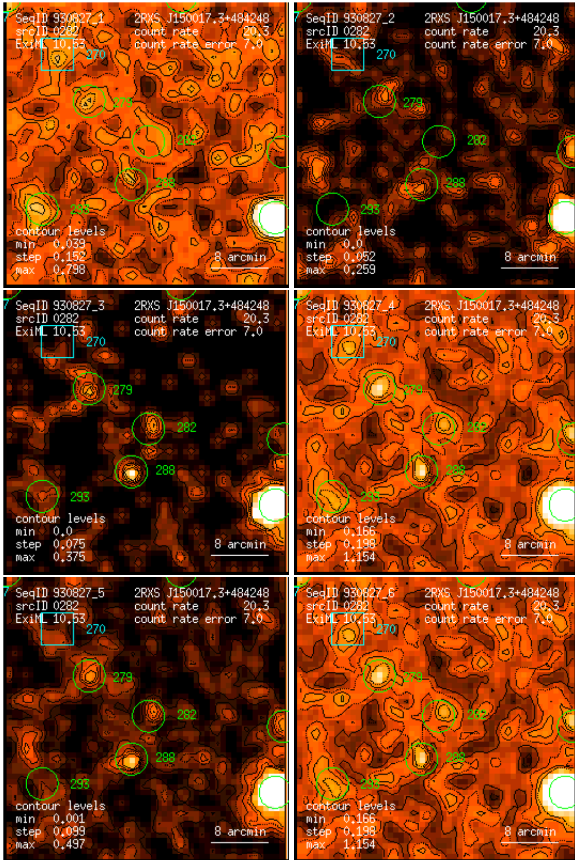
Figure 282: RASS 930827: detection 0282: band rate images, Gaussian filter: (1) PSPC channels 11 – 41, (2) 52 – 90, (3) 91 – 201, (4) 11 – 235, (5) 52 – 201, (6) 11 – 201. Broad band rates in counts/ks. Band rate contour levels in counts/ks/arcmin 2 .
