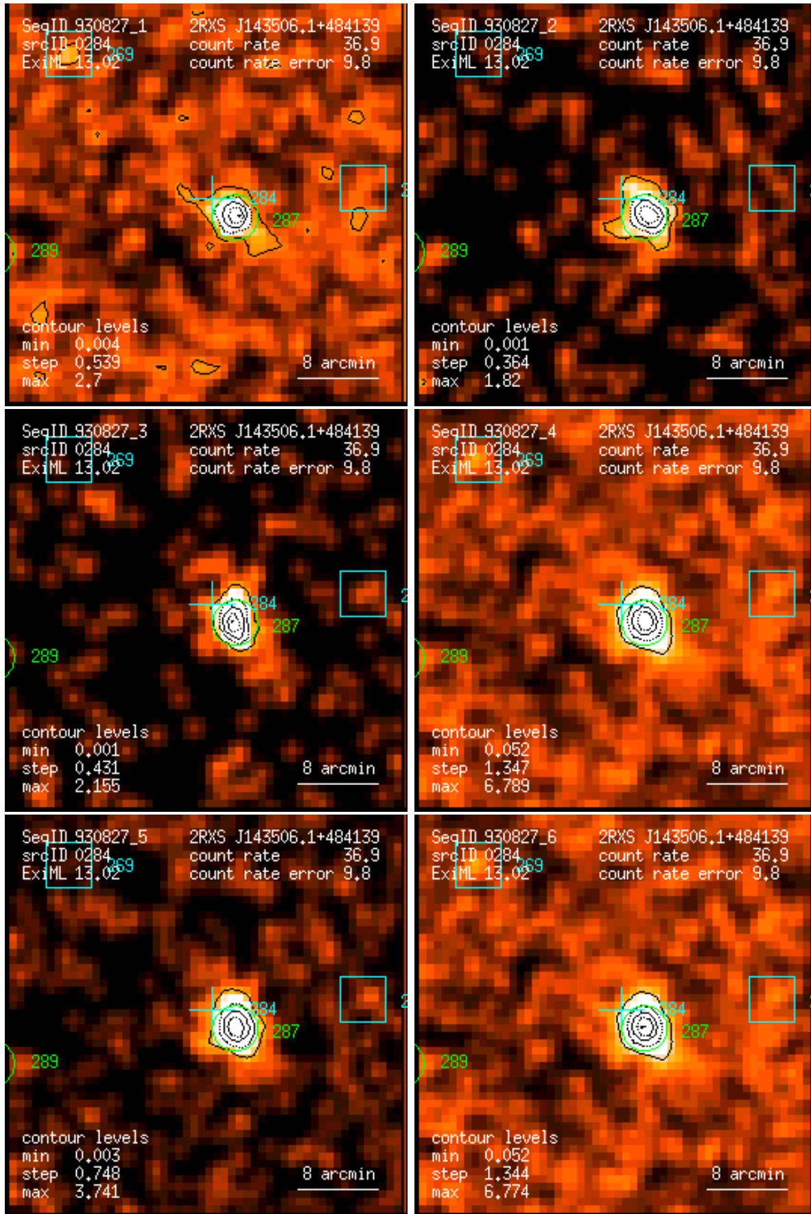
Figure 284: RASS 930827: detection 0284: band rate images, Gaussian filter: (1) PSPC channels 11 – 41, (2) 52 – 90, (3) 91 – 201, (4) 11 – 235, (5) 52 – 201, (6) 11 – 201. Broad band rates in counts/ks. Band rate contour levels in counts/ks/arcmin 2 .
