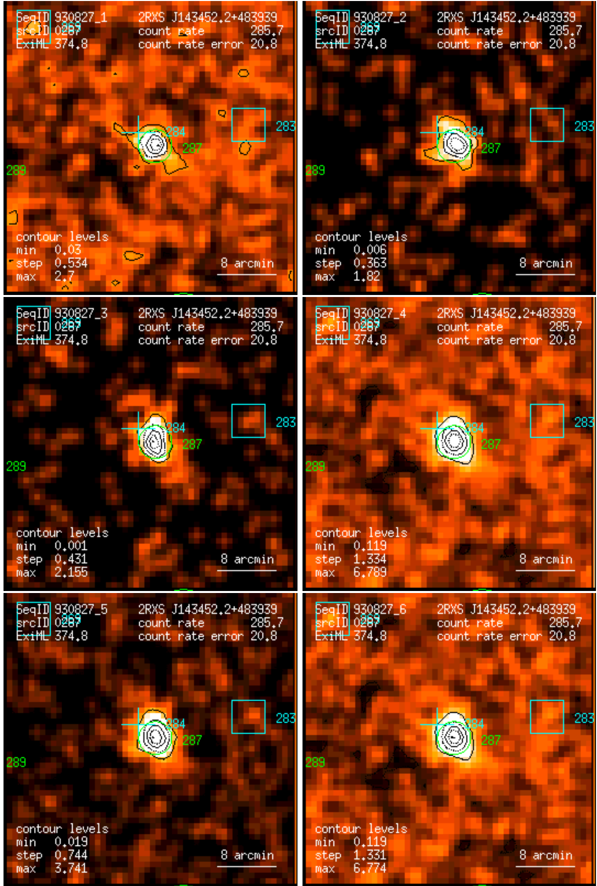
Figure 287: RASS 930827: detection 0287: band rate images, Gaussian filter: (1) PSPC channels 11 – 41, (2) 52 – 90, (3) 91 – 201, (4) 11 – 235, (5) 52 – 201, (6) 11 – 201. Broad band rates in counts/ks. Band rate contour levels in counts/ks/arcmin 2 .
