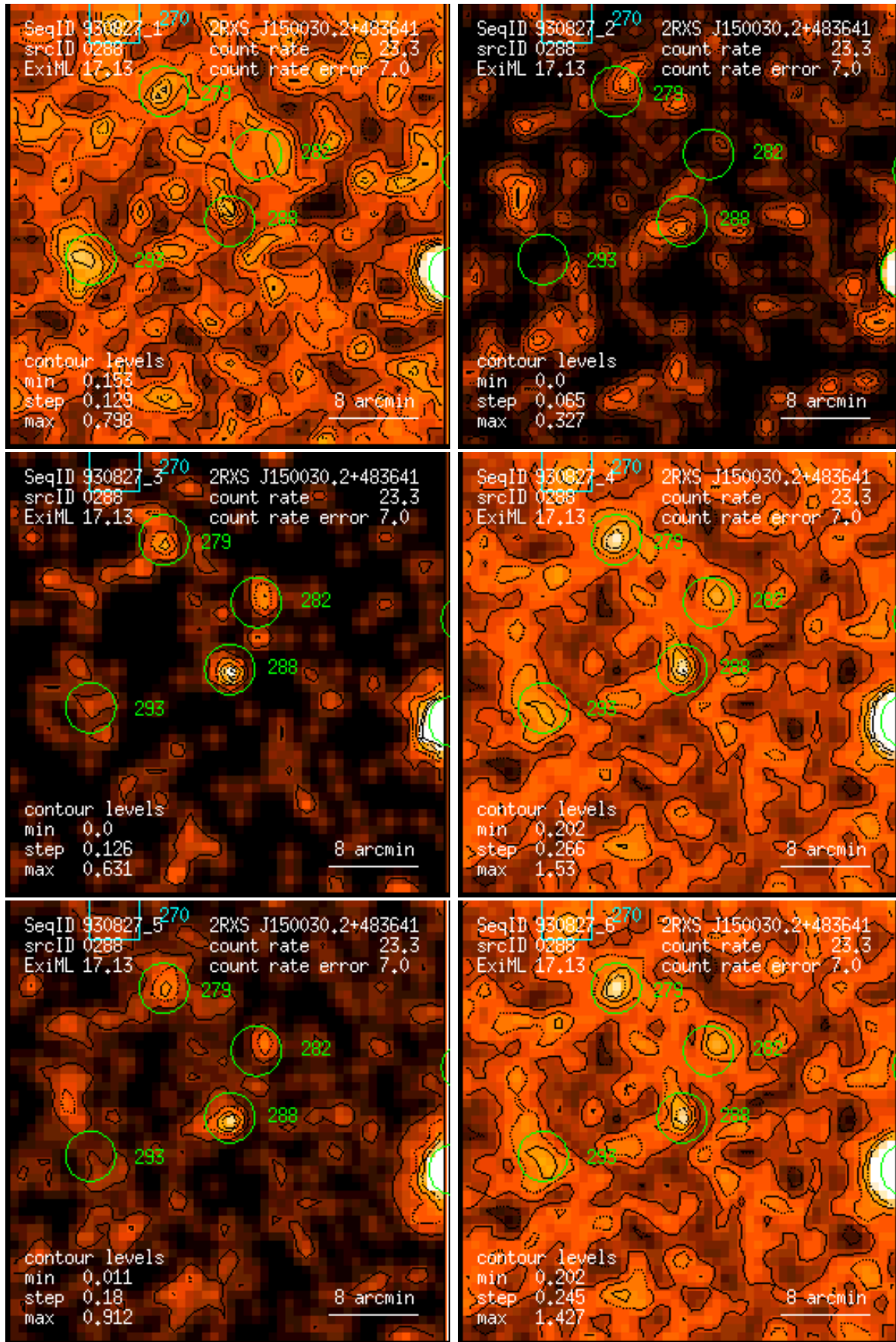
Figure 288: RASS 930827: detection 0288: band rate images, Gaussian filter: (1) PSPC channels 11 – 41, (2) 52 – 90, (3) 91 – 201, (4) 11 – 235, (5) 52 – 201, (6) 11 – 201. Broad band rates in counts/ks. Band rate contour levels in counts/ks/arcmin 2 .
