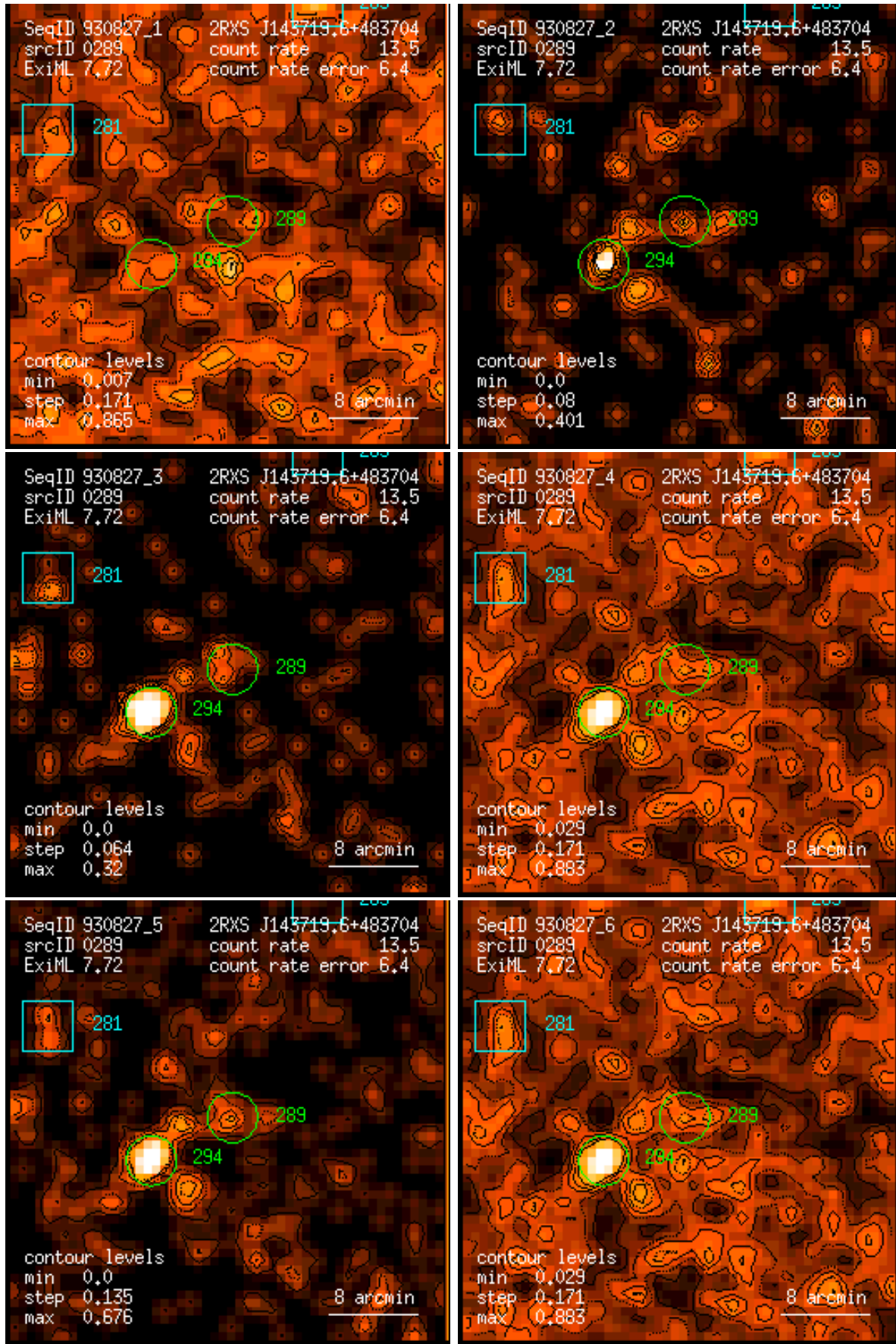
Figure 289: RASS 930827: detection 0289: band rate images, Gaussian filter: (1) PSPC channels 11 – 41, (2) 52 – 90, (3) 91 – 201, (4) 11 – 235, (5) 52 – 201, (6) 11 – 201. Broad band rates in counts/ks. Band rate contour levels in counts/ks/arcmin 2 .
