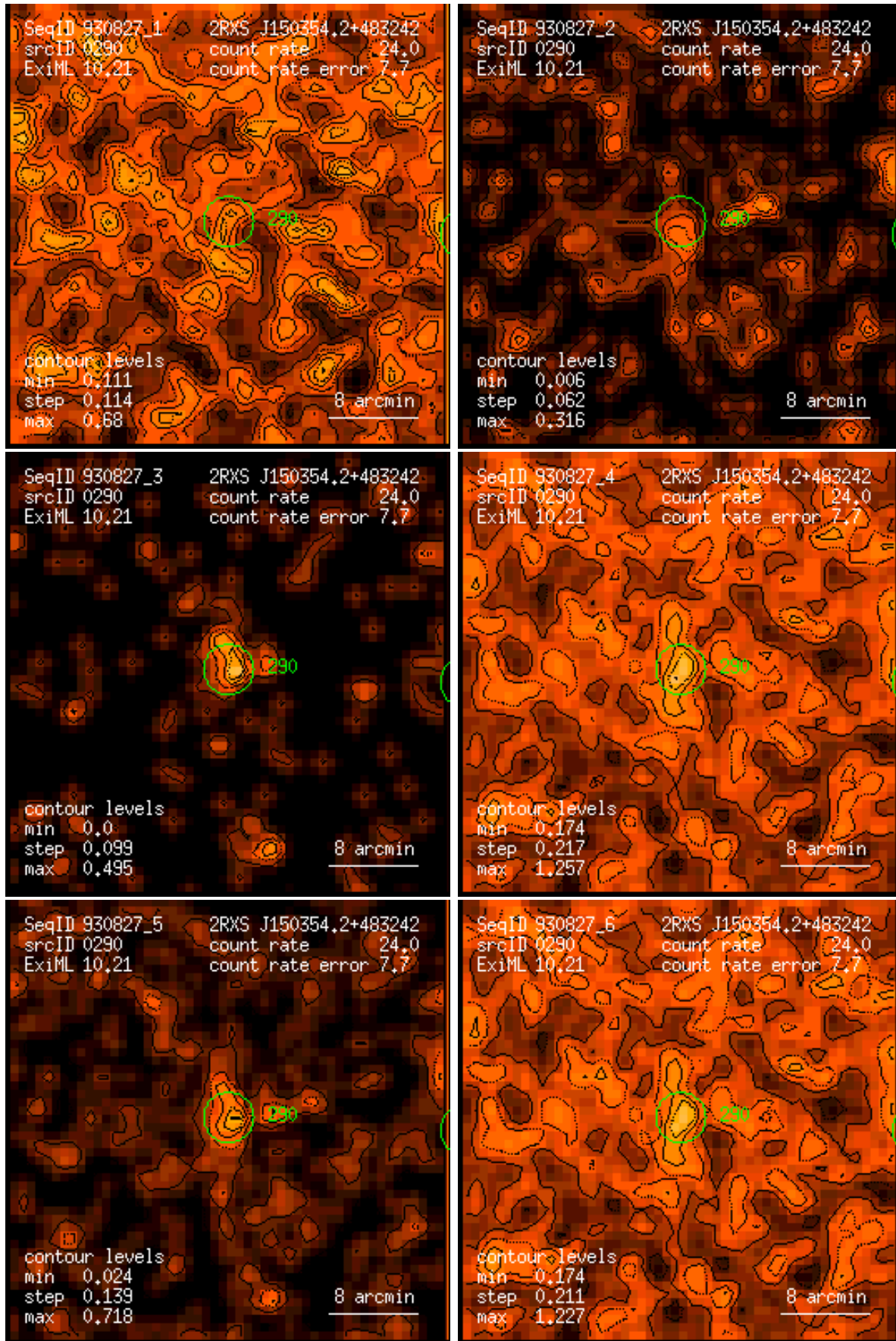
Figure 290: RASS 930827: detection 0290: band rate images, Gaussian filter: (1) PSPC channels 11 – 41, (2) 52 – 90, (3) 91 – 201, (4) 11 – 235, (5) 52 – 201, (6) 11 – 201. Broad band rates in counts/ks. Band rate contour levels in counts/ks/arcmin 2 .
