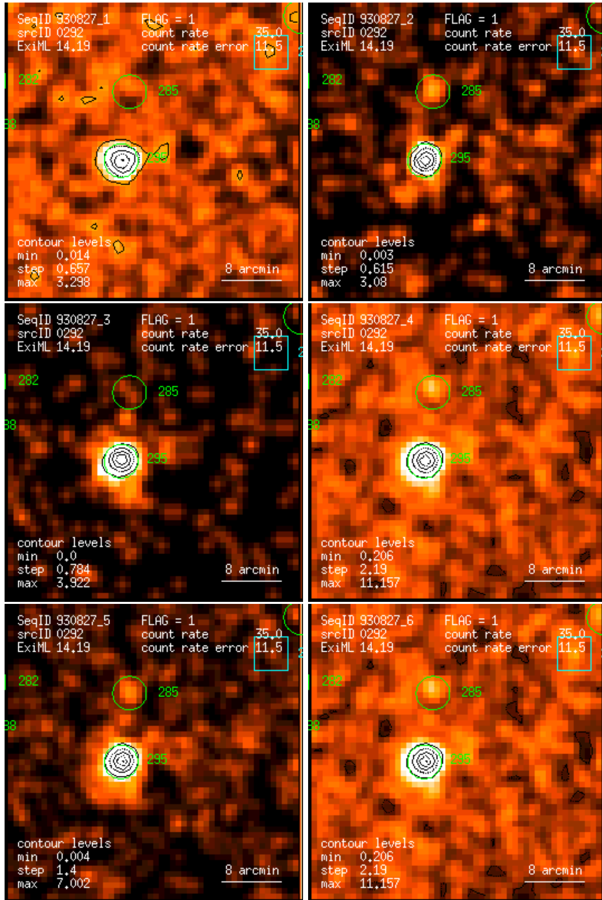
Figure 292: RASS 930827: detection 0292: band rate images, Gaussian filter: (1) PSPC channels 11 – 41, (2) 52 – 90, (3) 91 – 201, (4) 11 – 235, (5) 52 – 201, (6) 11 – 201. Broad band rates in counts/ks. Band rate contour levels in counts/ks/arcmin 2 .
