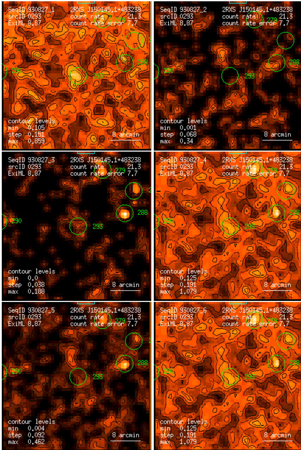
Figure 293: RASS 930827: detection 0293: band rate images, Gaussian filter: (1) PSPC channels 11 – 41, (2) 52 – 90, (3) 91 – 201, (4) 11 – 235, (5) 52 – 201, (6) 11 – 201. Broad band rates in counts/ks. Band rate contour levels in counts/ks/arcmin 2 .
