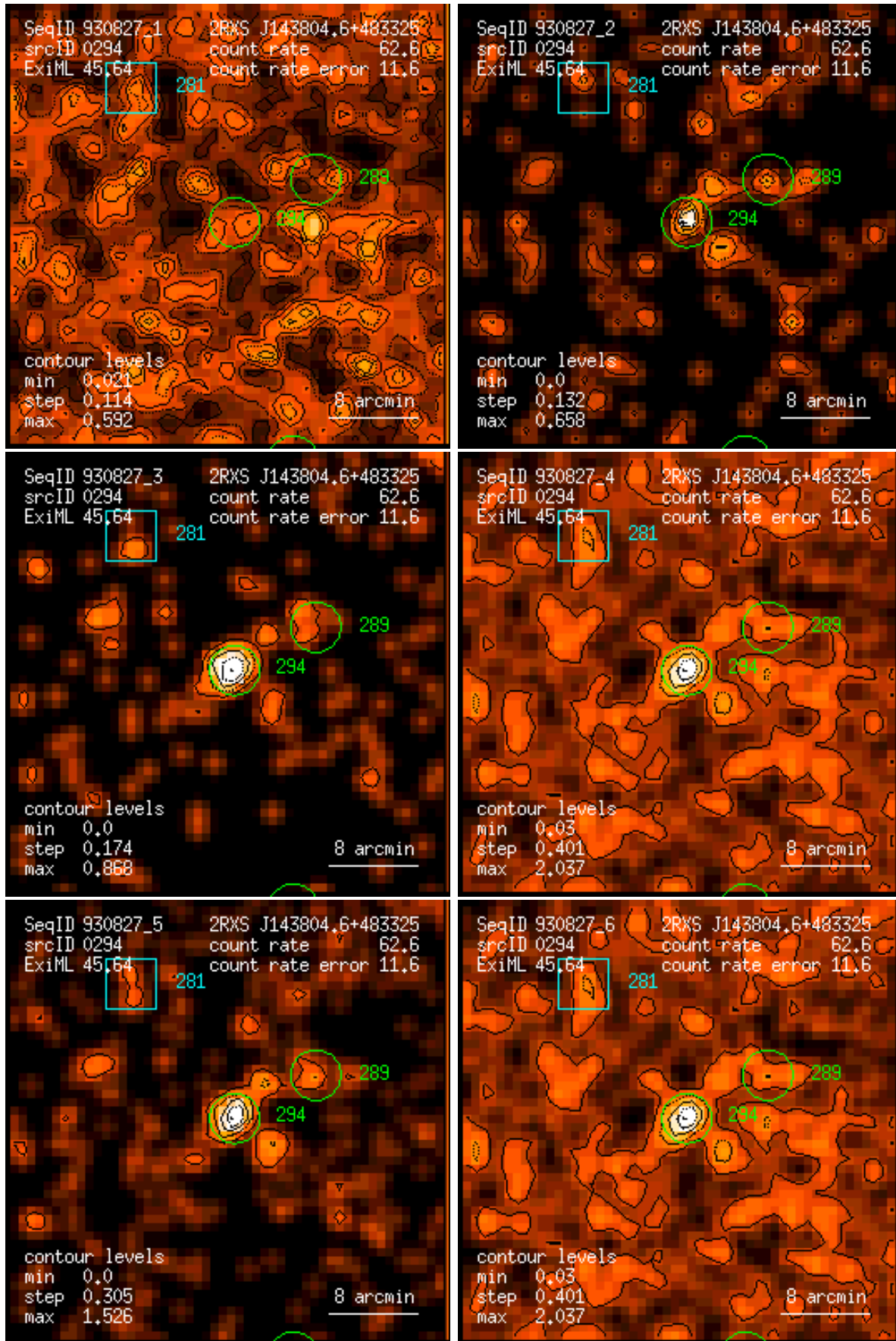
Figure 294: RASS 930827: detection 0294: band rate images, Gaussian filter: (1) PSPC channels 11 – 41, (2) 52 – 90, (3) 91 – 201, (4) 11 – 235, (5) 52 – 201, (6) 11 – 201. Broad band rates in counts/ks. Band rate contour levels in counts/ks/arcmin 2 .
