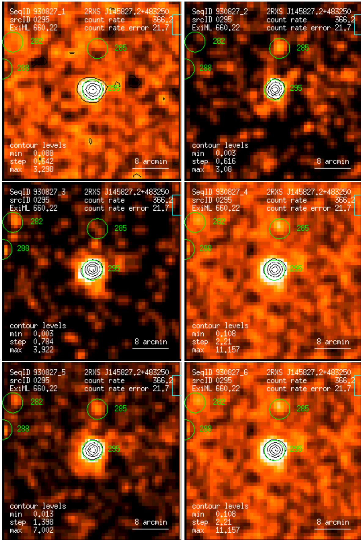
Figure 295: RASS 930827: detection 0295: band rate images, Gaussian filter: (1) PSPC channels 11 – 41, (2) 52 – 90, (3) 91 – 201, (4) 11 – 235, (5) 52 – 201, (6) 11 – 201. Broad band rates in counts/ks. Band rate contour levels in counts/ks/arcmin 2 .
