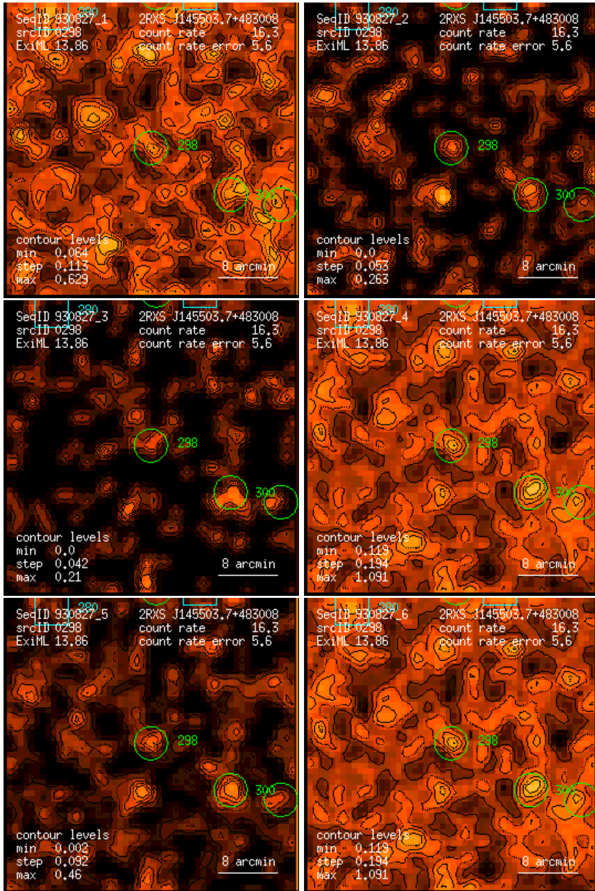
Figure 298: RASS 930827: detection 0298: band rate images, Gaussian filter: (1) PSPC channels 11 – 41, (2) 52 – 90, (3) 91 – 201, (4) 11 – 235, (5) 52 – 201, (6) 11 – 201. Broad band rates in counts/ks. Band rate contour levels in counts/ks/arcmin 2 .
