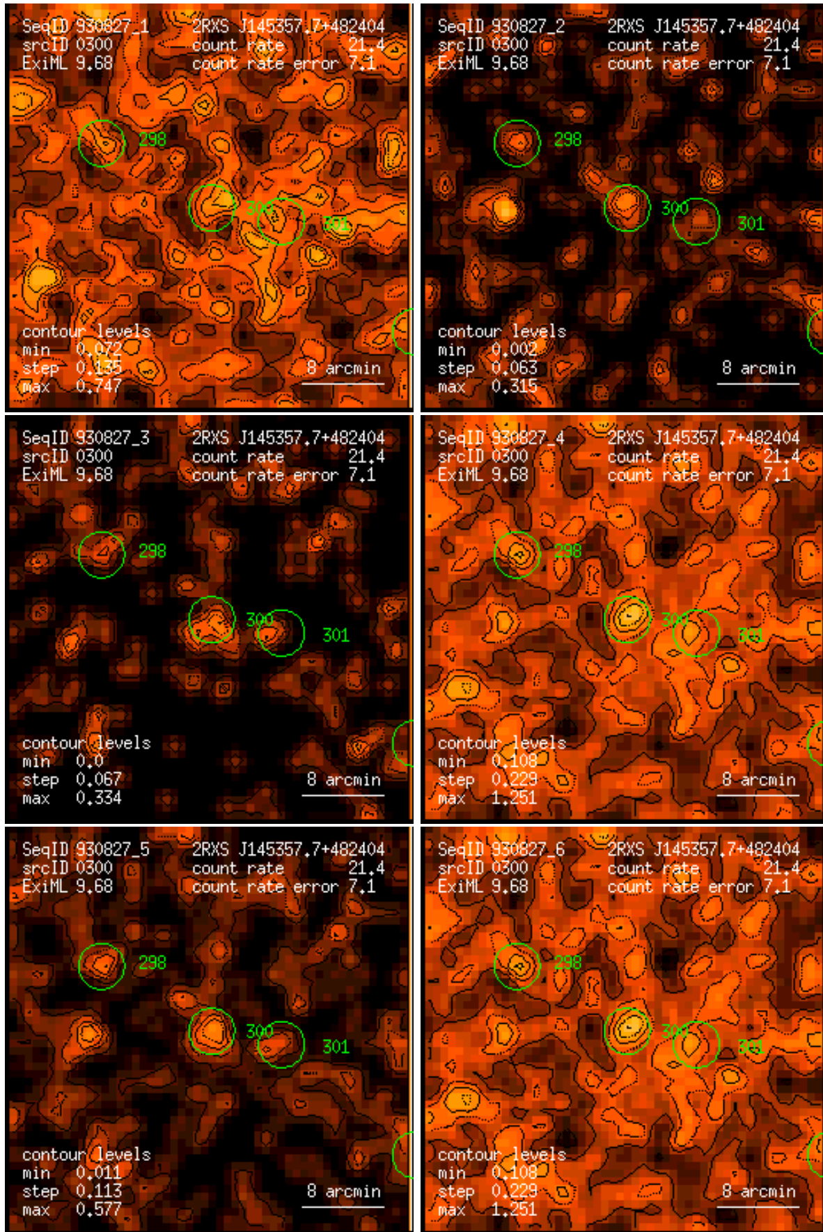
Figure 300: RASS 930827: detection 0300: band rate images, Gaussian filter: (1) PSPC channels 11 – 41, (2) 52 – 90, (3) 91 – 201, (4) 11 – 235, (5) 52 – 201, (6) 11 – 201. Broad band rates in counts/ks. Band rate contour levels in counts/ks/arcmin 2 .
