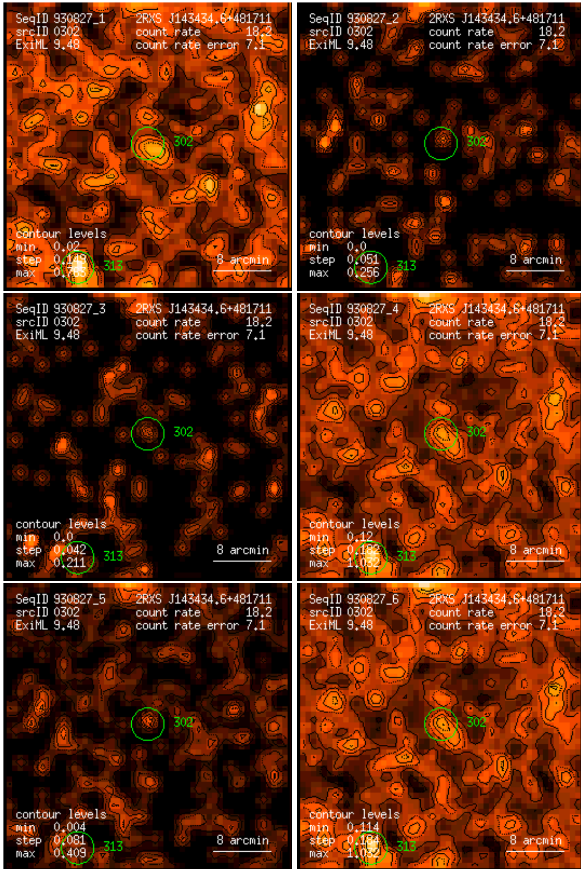
Figure 302: RASS 930827: detection 0302: band rate images, Gaussian filter: (1) PSPC channels 11 – 41, (2) 52 – 90, (3) 91 – 201, (4) 11 – 235, (5) 52 – 201, (6) 11 – 201. Broad band rates in counts/ks. Band rate contour levels in counts/ks/arcmin 2 .
