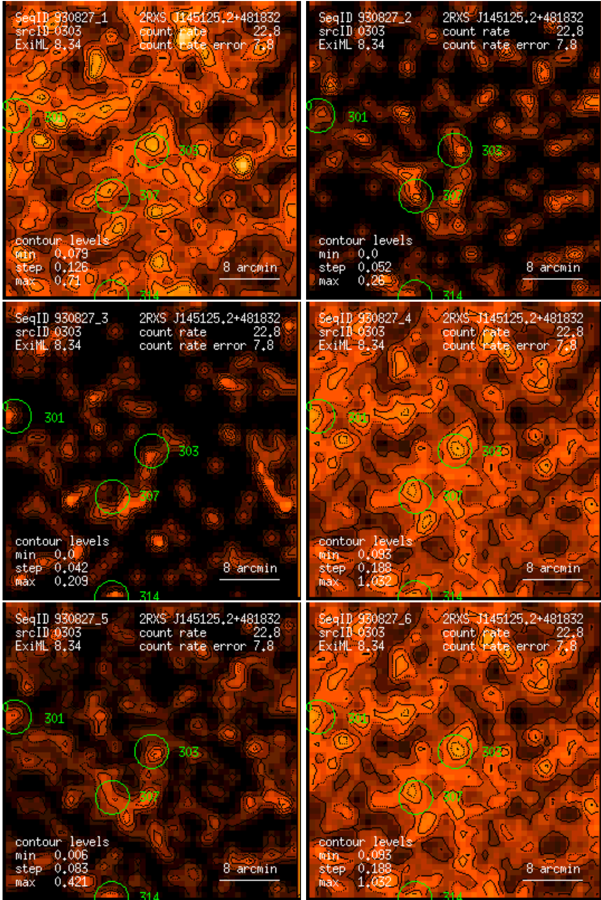
Figure 303: RASS 930827: detection 0303: band rate images, Gaussian filter: (1) PSPC channels 11 – 41, (2) 52 – 90, (3) 91 – 201, (4) 11 – 235, (5) 52 – 201, (6) 11 – 201. Broad band rates in counts/ks. Band rate contour levels in counts/ks/arcmin 2 .
