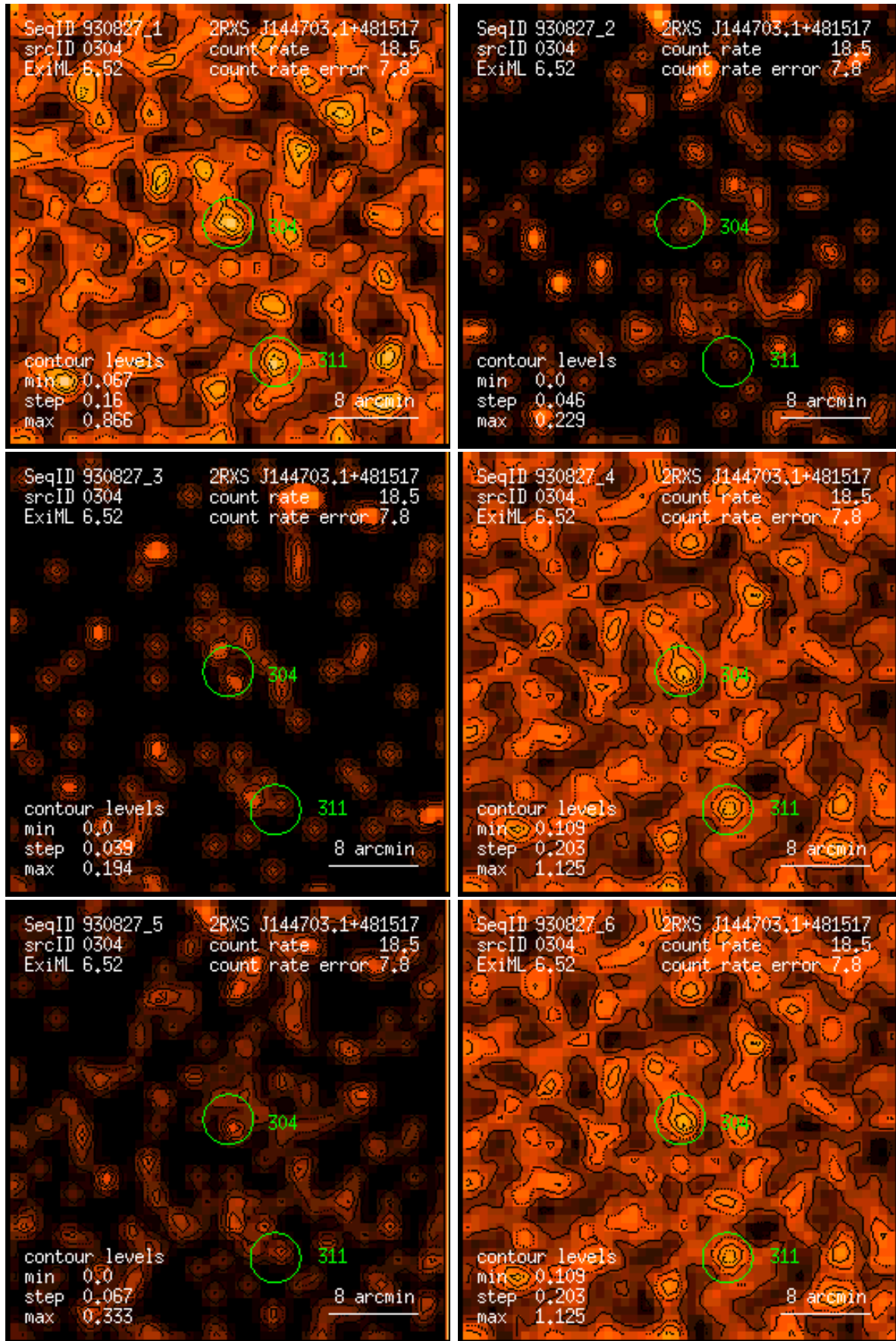
Figure 304: RASS 930827: detection 0304: band rate images, Gaussian filter: (1) PSPC channels 11 – 41, (2) 52 – 90, (3) 91 – 201, (4) 11 – 235, (5) 52 – 201, (6) 11 – 201. Broad band rates in counts/ks. Band rate contour levels in counts/ks/arcmin 2 .
