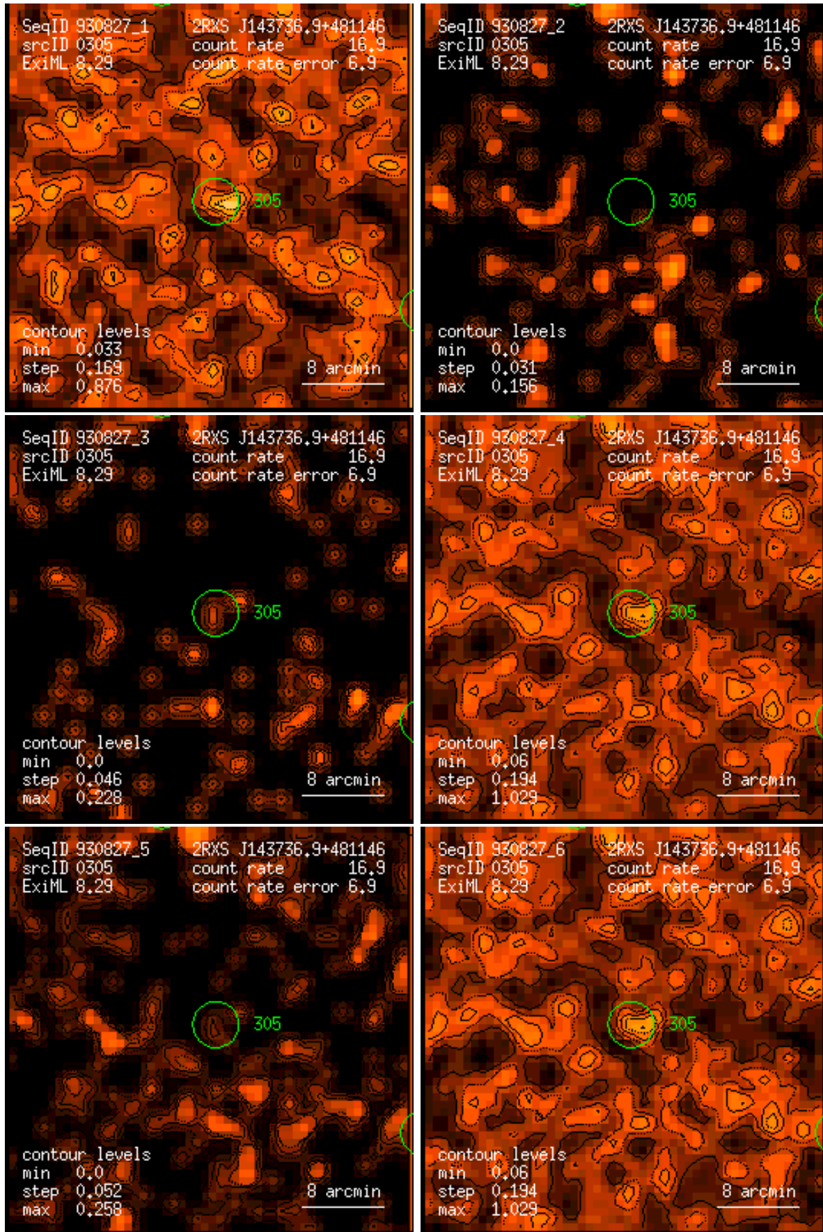
Figure 305: RASS 930827: detection 0305: band rate images, Gaussian filter: (1) PSPC channels 11 – 41, (2) 52 – 90, (3) 91 – 201, (4) 11 – 235, (5) 52 – 201, (6) 11 – 201. Broad band rates in counts/ks. Band rate contour levels in counts/ks/arcmin 2 .
