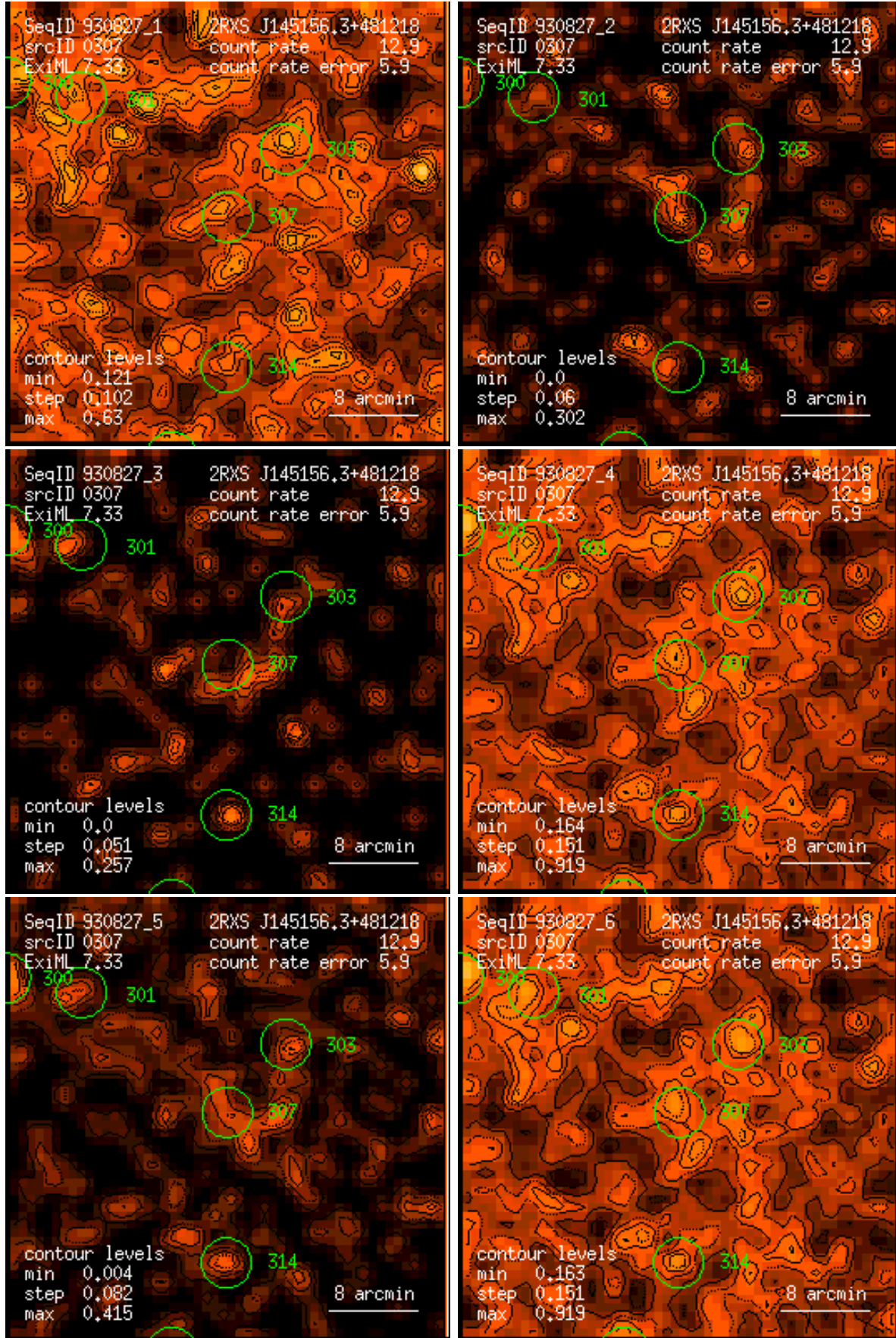
Figure 307: RASS 930827: detection 0307: band rate images, Gaussian filter: (1) PSPC channels 11 – 41, (2) 52 – 90, (3) 91 – 201, (4) 11 – 235, (5) 52 – 201, (6) 11 – 201. Broad band rates in counts/ks. Band rate contour levels in counts/ks/arcmin 2 .
