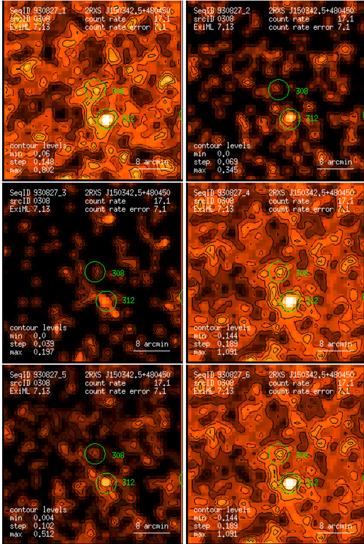
Figure 308: RASS 930827: detection 0308: band rate images, Gaussian filter: (1) PSPC channels 11 – 41, (2) 52 – 90, (3) 91 – 201, (4) 11 – 235, (5) 52 – 201, (6) 11 – 201. Broad band rates in counts/ks. Band rate contour levels in counts/ks/arcmin 2 .
