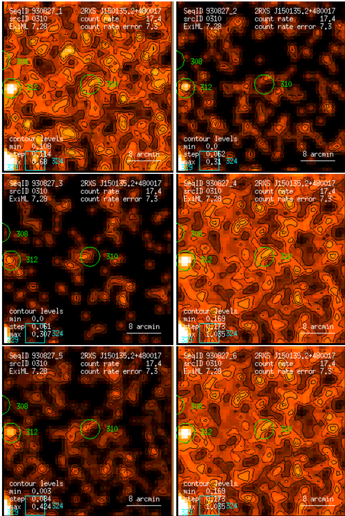
Figure 310: RASS 930827: detection 0310: band rate images, Gaussian filter: (1) PSPC channels 11 – 41, (2) 52 – 90, (3) 91 – 201, (4) 11 – 235, (5) 52 – 201, (6) 11 – 201. Broad band rates in counts/ks. Band rate contour levels in counts/ks/arcmin 2 .
