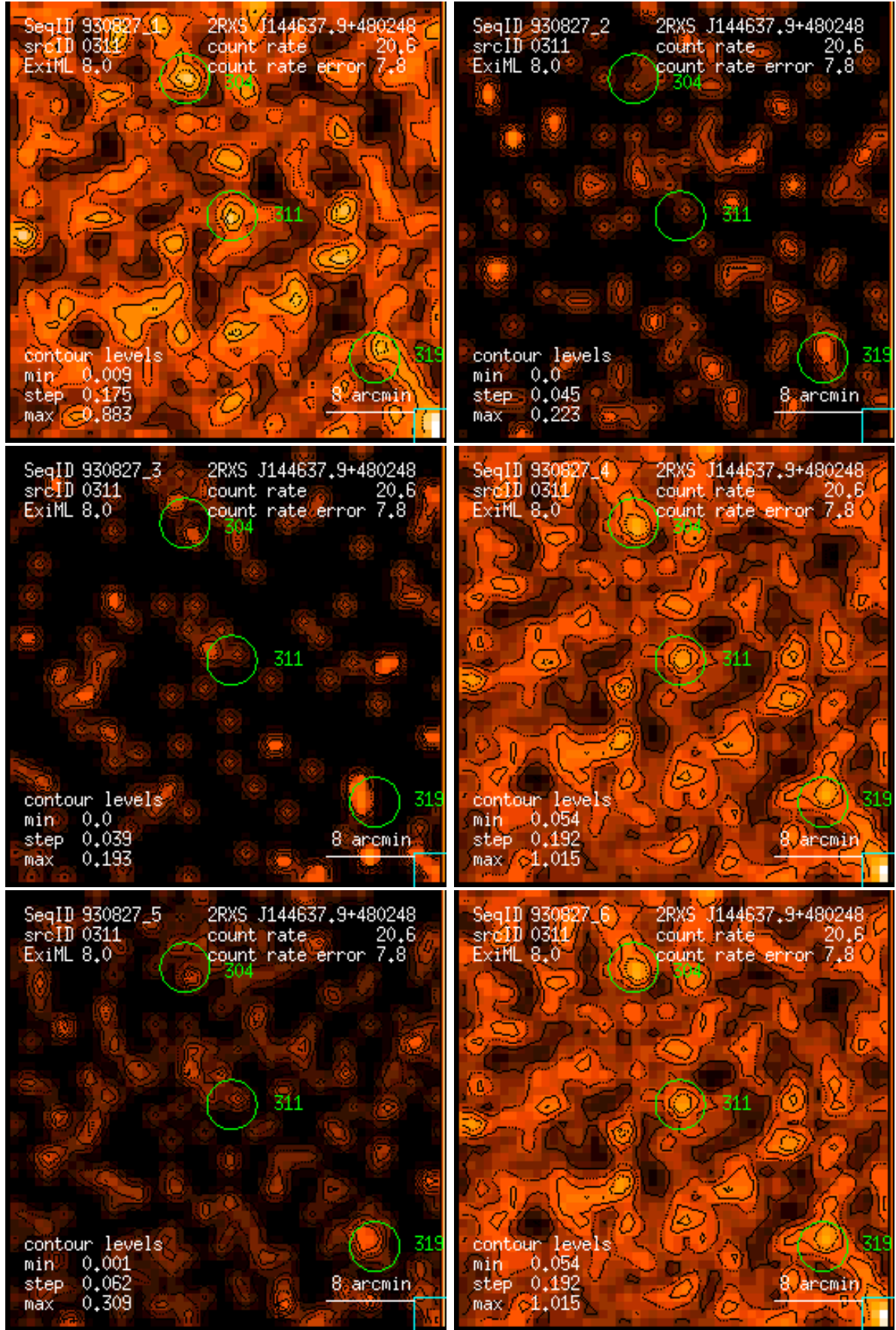
Figure 311: RASS 930827: detection 0311: band rate images, Gaussian filter: (1) PSPC channels 11 – 41, (2) 52 – 90, (3) 91 – 201, (4) 11 – 235, (5) 52 – 201, (6) 11 – 201. Broad band rates in counts/ks. Band rate contour levels in counts/ks/arcmin 2 .
