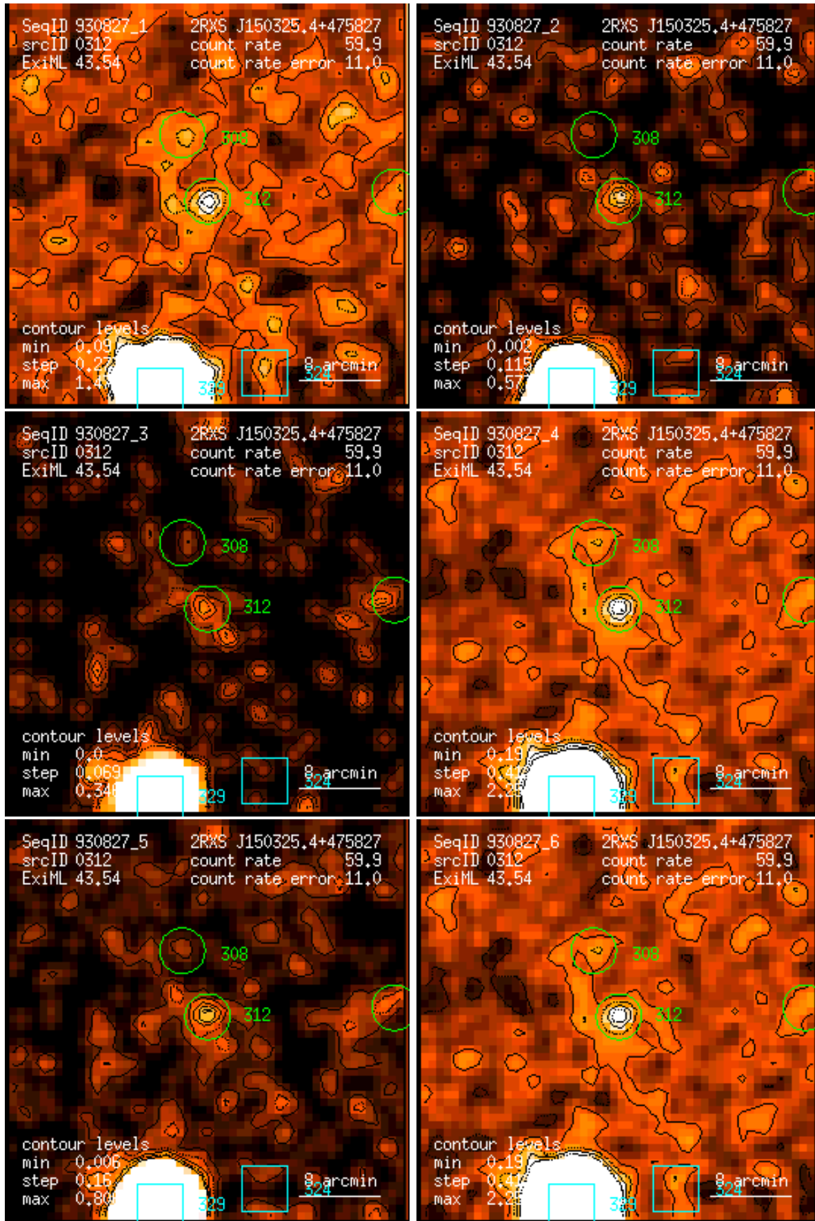
Figure 312: RASS 930827: detection 0312: band rate images, Gaussian filter: (1) PSPC channels 11 – 41, (2) 52 – 90, (3) 91 – 201, (4) 11 – 235, (5) 52 – 201, (6) 11 – 201. Broad band rates in counts/ks. Band rate contour levels in counts/ks/arcmin 2 .
