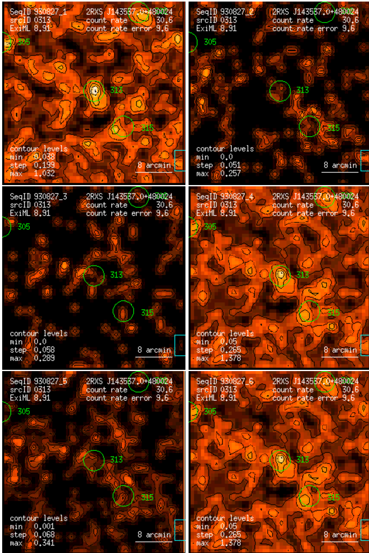
Figure 313: RASS 930827: detection 0313: band rate images, Gaussian filter: (1) PSPC channels 11 – 41, (2) 52 – 90, (3) 91 – 201, (4) 11 – 235, (5) 52 – 201, (6) 11 – 201. Broad band rates in counts/ks. Band rate contour levels in counts/ks/arcmin 2 .
