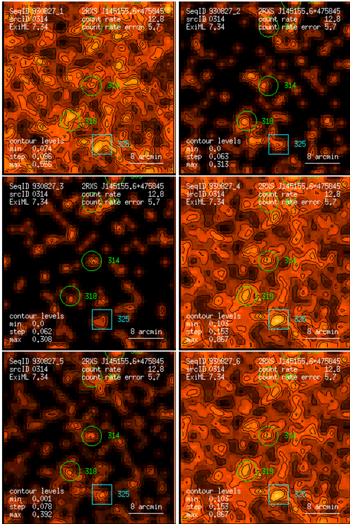
Figure 314: RASS 930827: detection 0314: band rate images, Gaussian filter: (1) PSPC channels 11 – 41, (2) 52 – 90, (3) 91 – 201, (4) 11 – 235, (5) 52 – 201, (6) 11 – 201. Broad band rates in counts/ks. Band rate contour levels in counts/ks/arcmin 2 .
