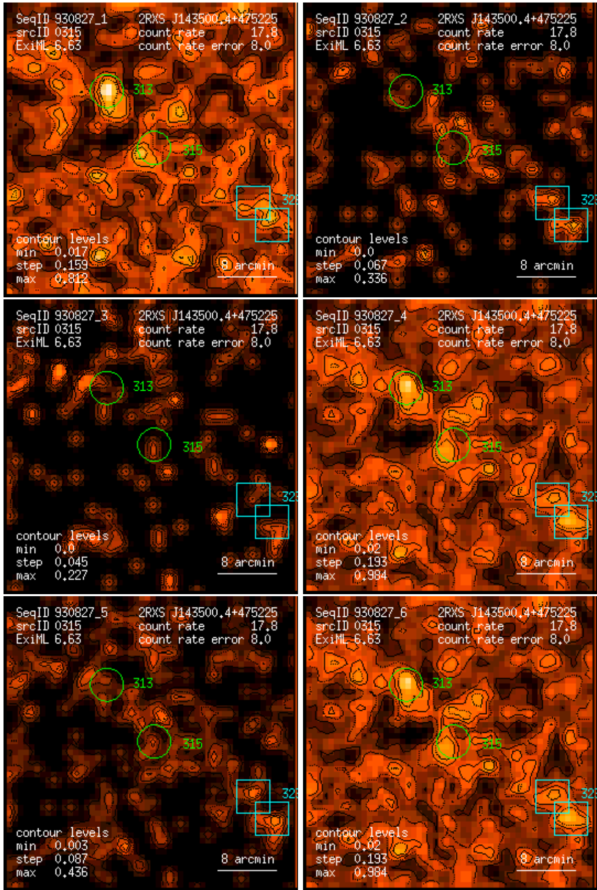
Figure 315: RASS 930827: detection 0315: band rate images, Gaussian filter: (1) PSPC channels 11 – 41, (2) 52 – 90, (3) 91 – 201, (4) 11 – 235, (5) 52 – 201, (6) 11 – 201. Broad band rates in counts/ks. Band rate contour levels in counts/ks/arcmin 2 .
