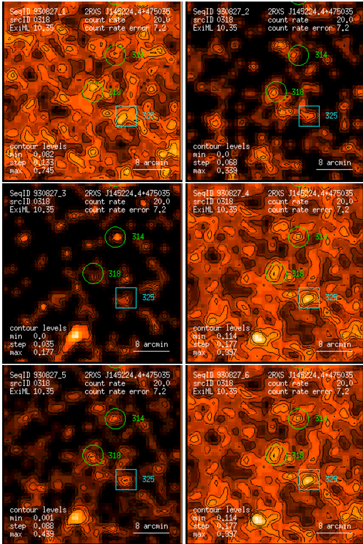
Figure 318: RASS 930827: detection 0318: band rate images, Gaussian filter: (1) PSPC channels 11 – 41, (2) 52 – 90, (3) 91 – 201, (4) 11 – 235, (5) 52 – 201, (6) 11 – 201. Broad band rates in counts/ks. Band rate contour levels in counts/ks/arcmin 2 .
