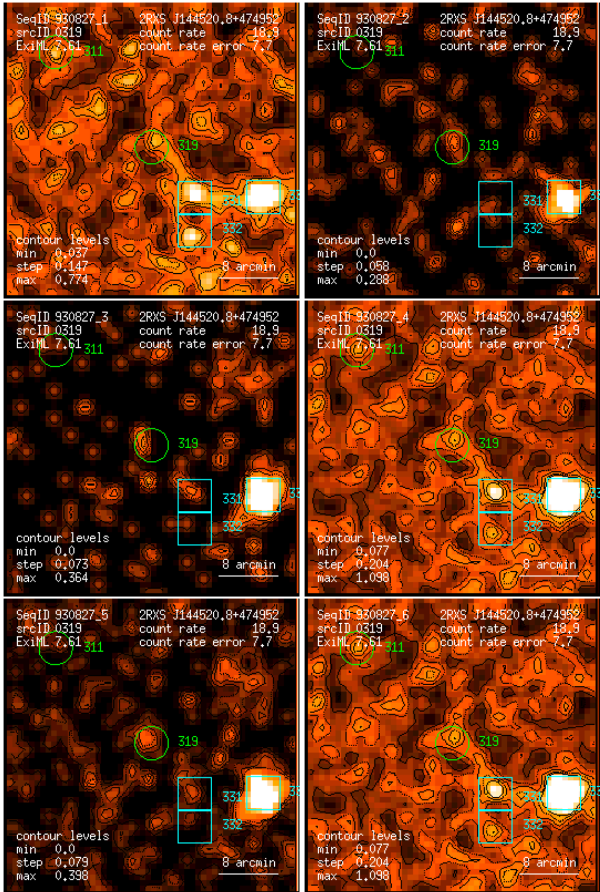
Figure 319: RASS 930827: detection 0319: band rate images, Gaussian filter: (1) PSPC channels 11 – 41, (2) 52 – 90, (3) 91 – 201, (4) 11 – 235, (5) 52 – 201, (6) 11 – 201. Broad band rates in counts/ks. Band rate contour levels in counts/ks/arcmin 2 .
