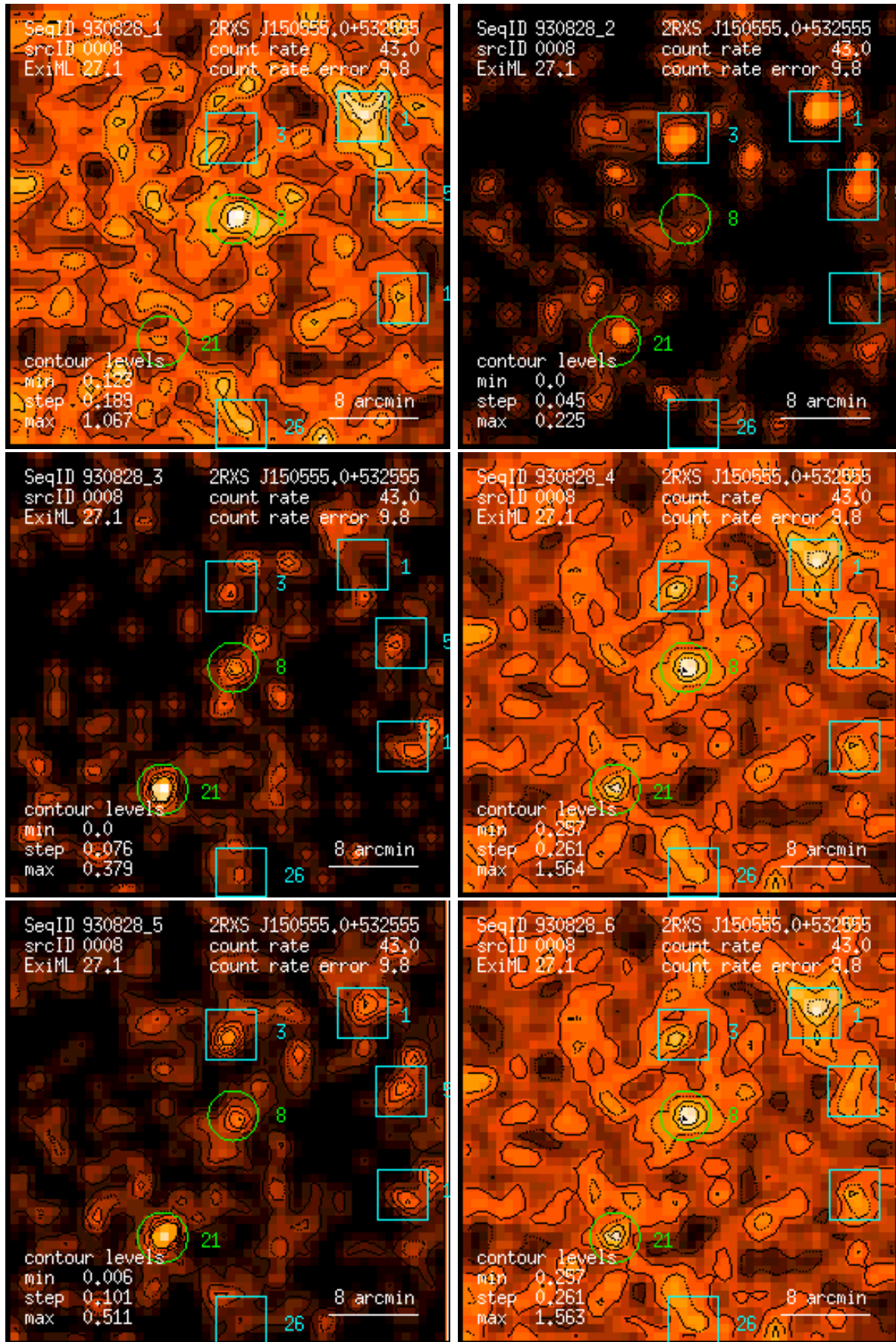
Figure 8: RASS 930828: detection 0008: band rate images, Gaussian filter: (1) PSPC channels 11 – 41, (2) 52 – 90, (3) 91 – 201, (4) 11 – 235, (5) 52 – 201, (6) 11 – 201. Broad band rates in counts/ks. Band rate contour levels in counts/ks/arcmin 2 .
